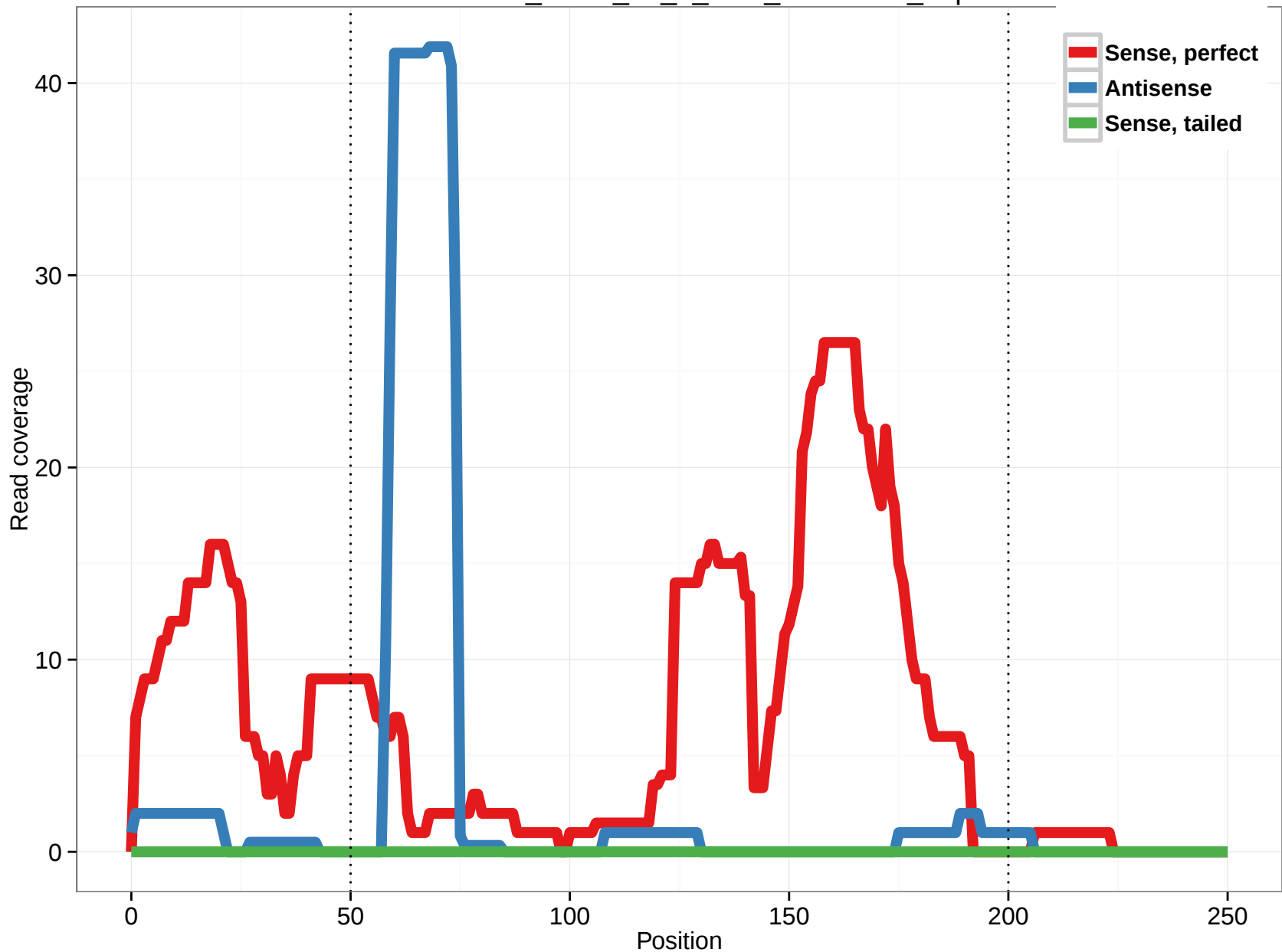
uc003his.2_intron_10_0_chr4_76587234_r.5p
