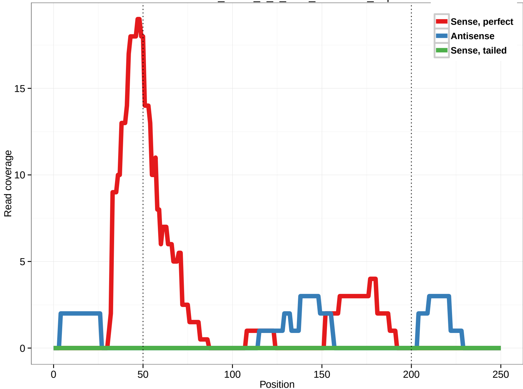
uc003hfs.2_intron_8_0_chr4_71702032_r.5p
