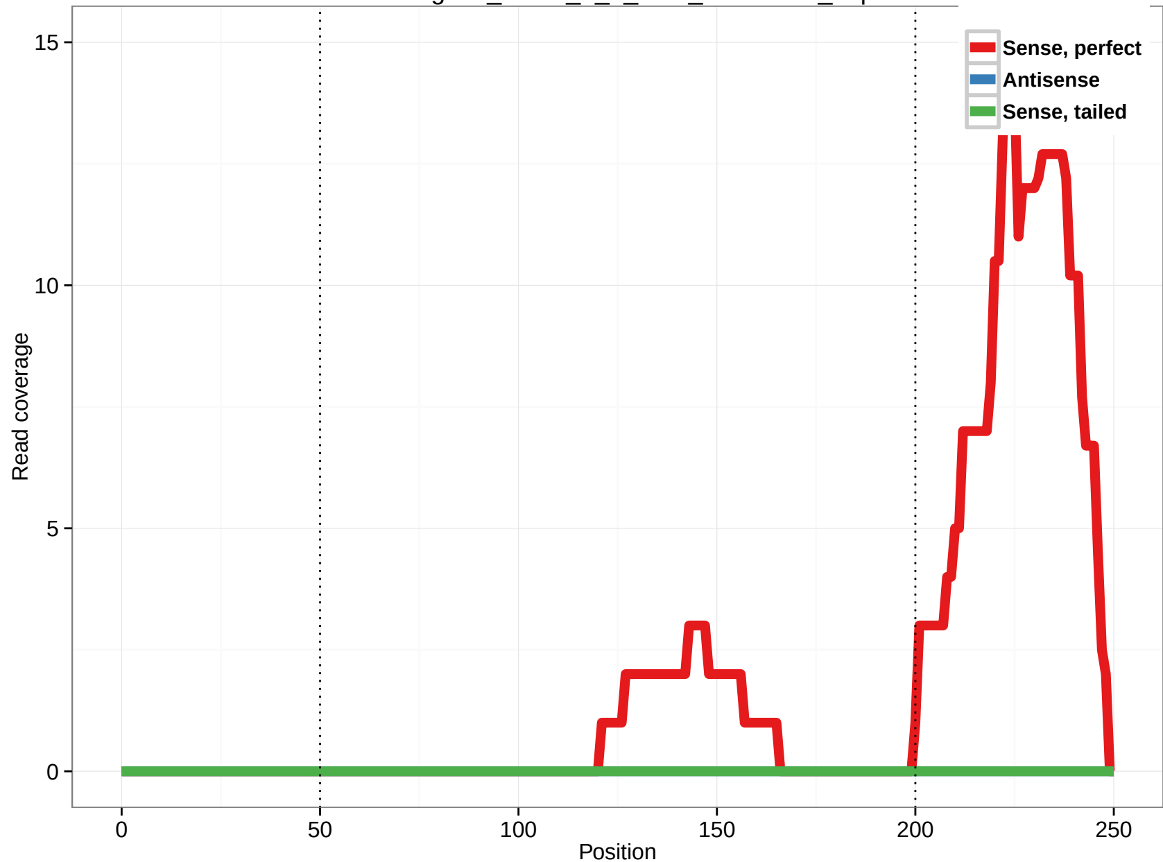
uc003gni.1_intron_5_0_chr4_15054209_f.3p
