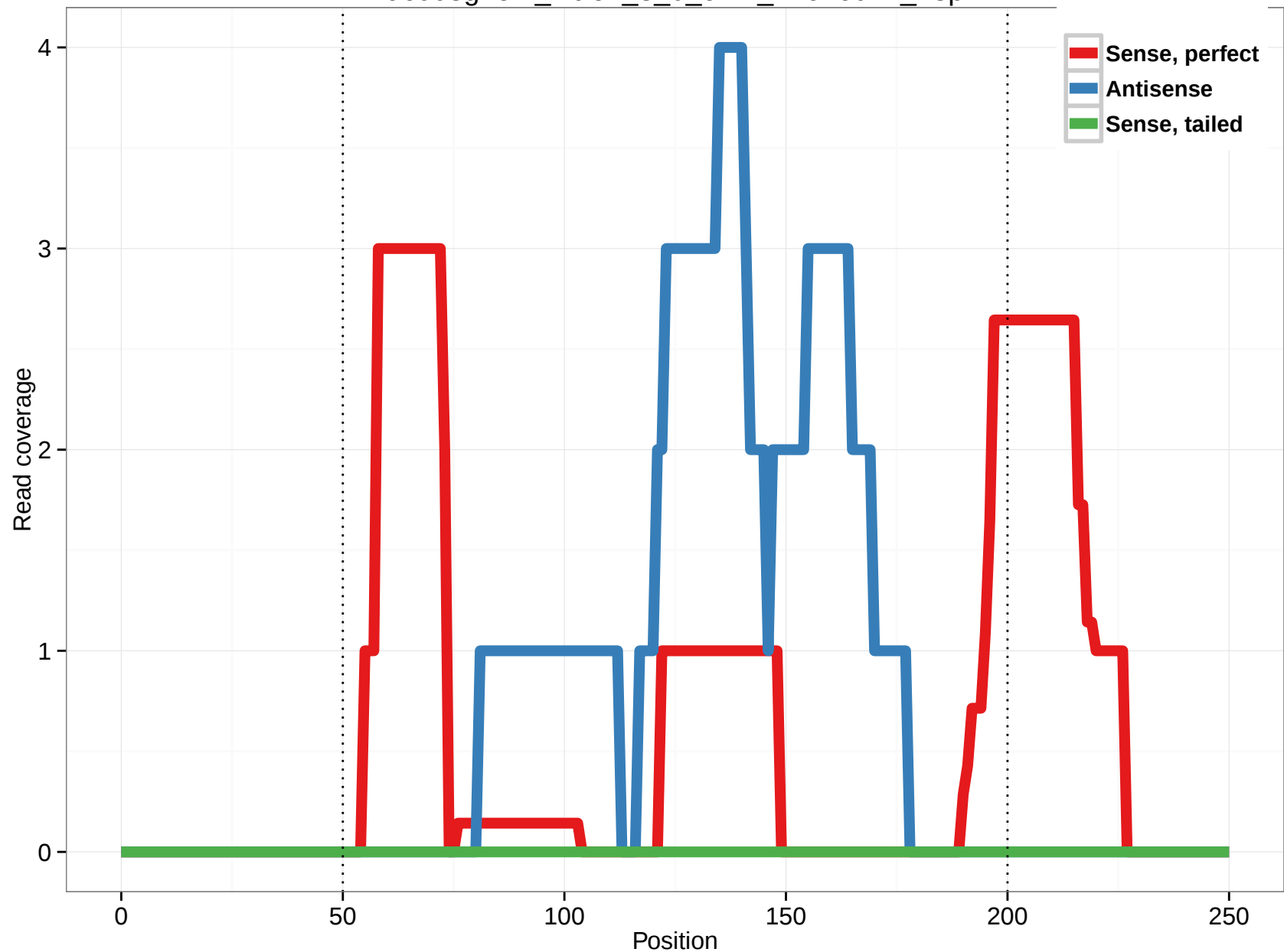
uc003gne.2_intron_3_0_chr4_14616041_r.3p
