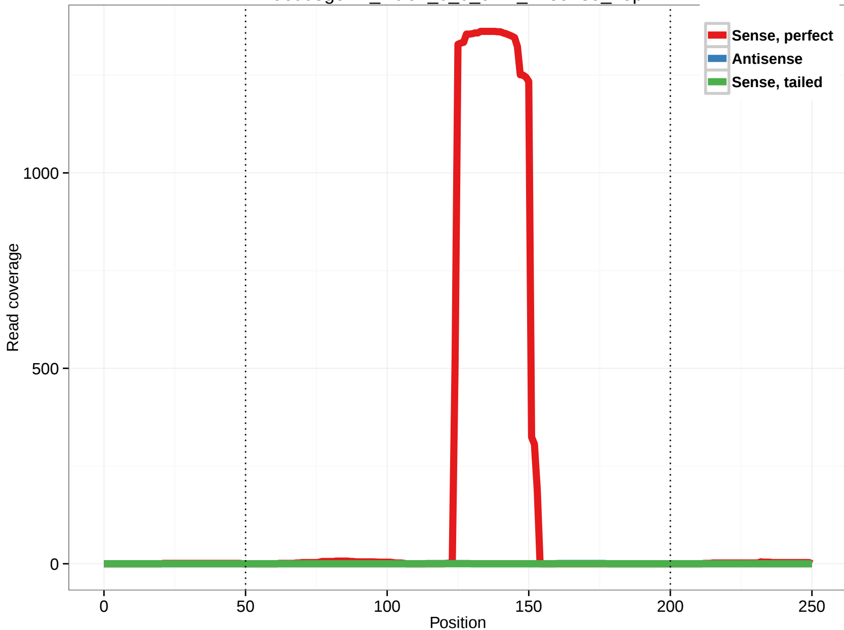
uc003gev.1_intron_0_0_chr4_2259739_r.5p
