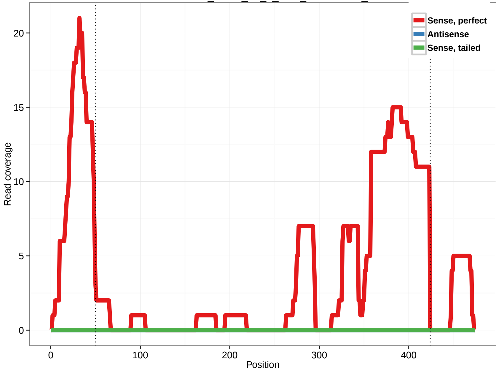
uc003fvz.3_intron_10_0_chr3_195794529_r
