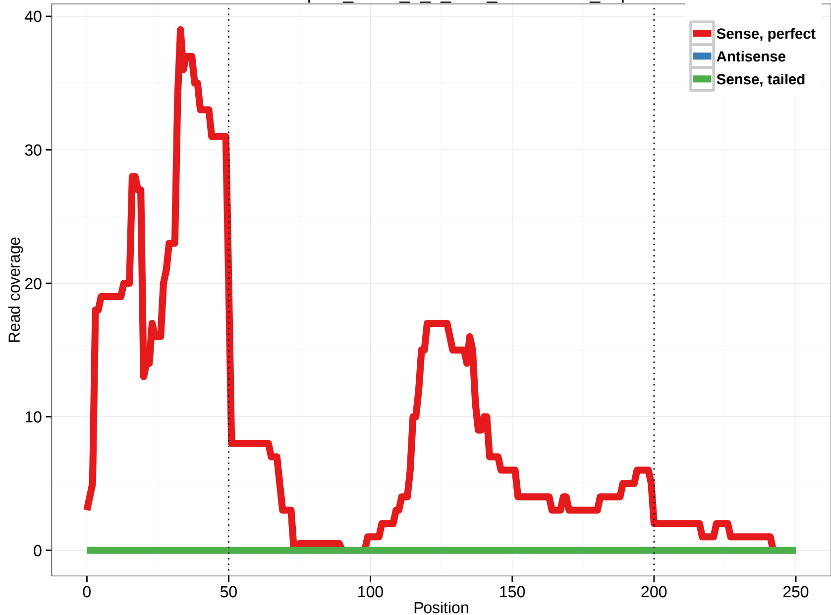
uc003fpu.2_intron_6_0_chr3_185643415_r.5p
