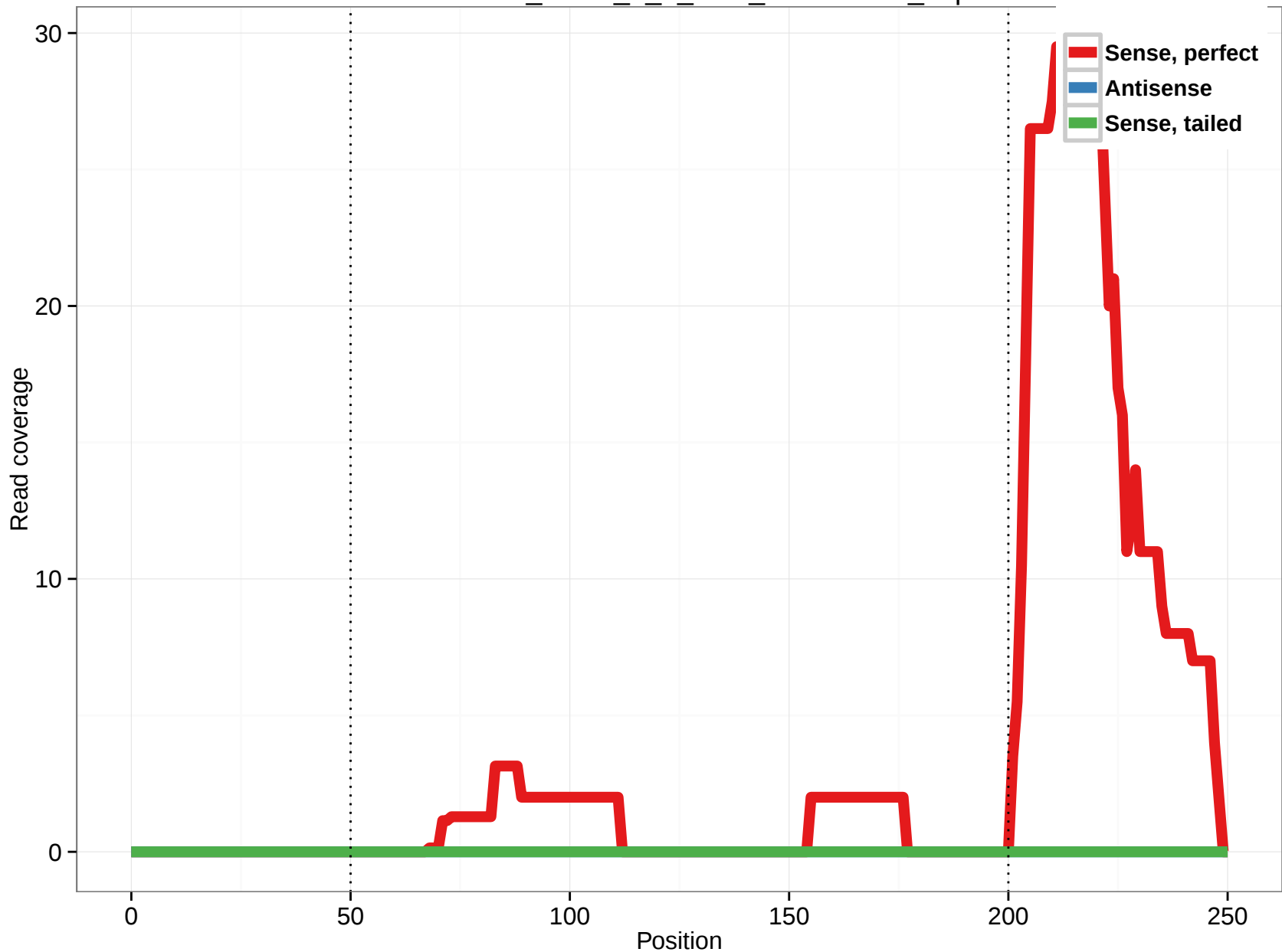
uc003fkc.2_intron_4_0_chr3_179336310_f.3p
