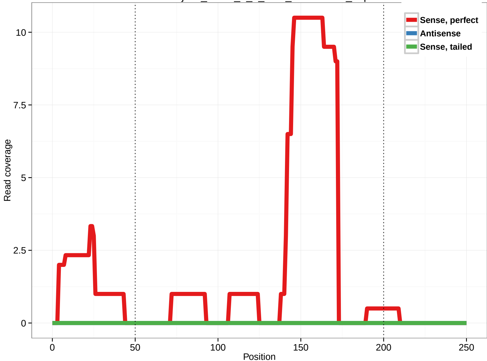
uc003fjw.2_intron_2_0_chr3_179288030_f.5p
