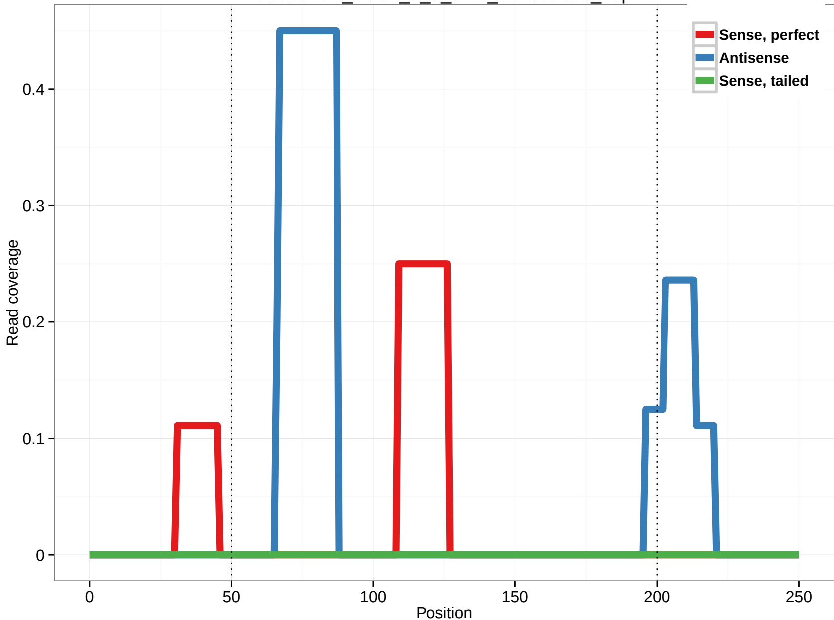
uc003ffc.2_intron_3_0_chr3_167630693_f.5p
