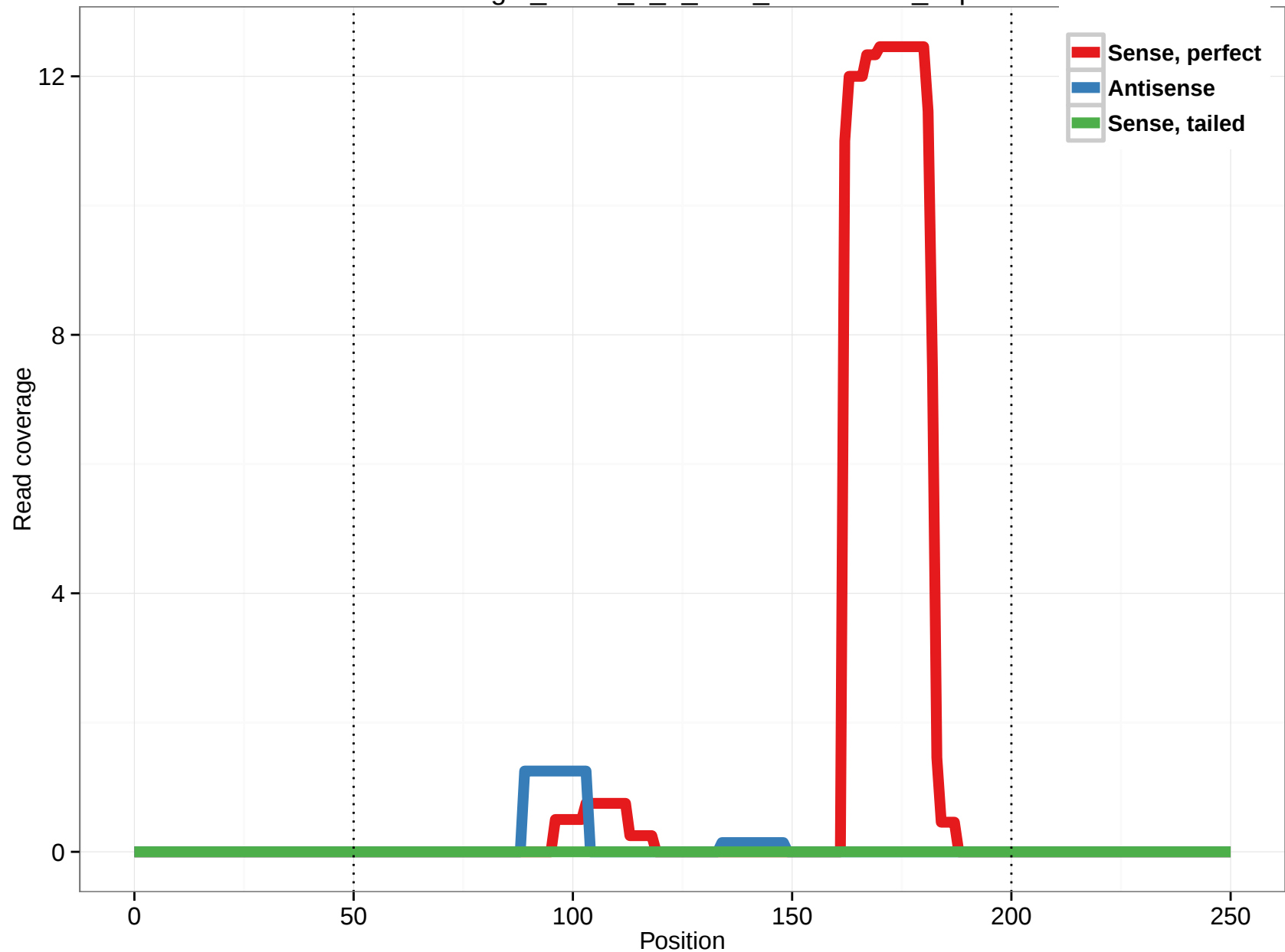
uc003feg.2_intron_2_0_chr3_162632023_f.3p
