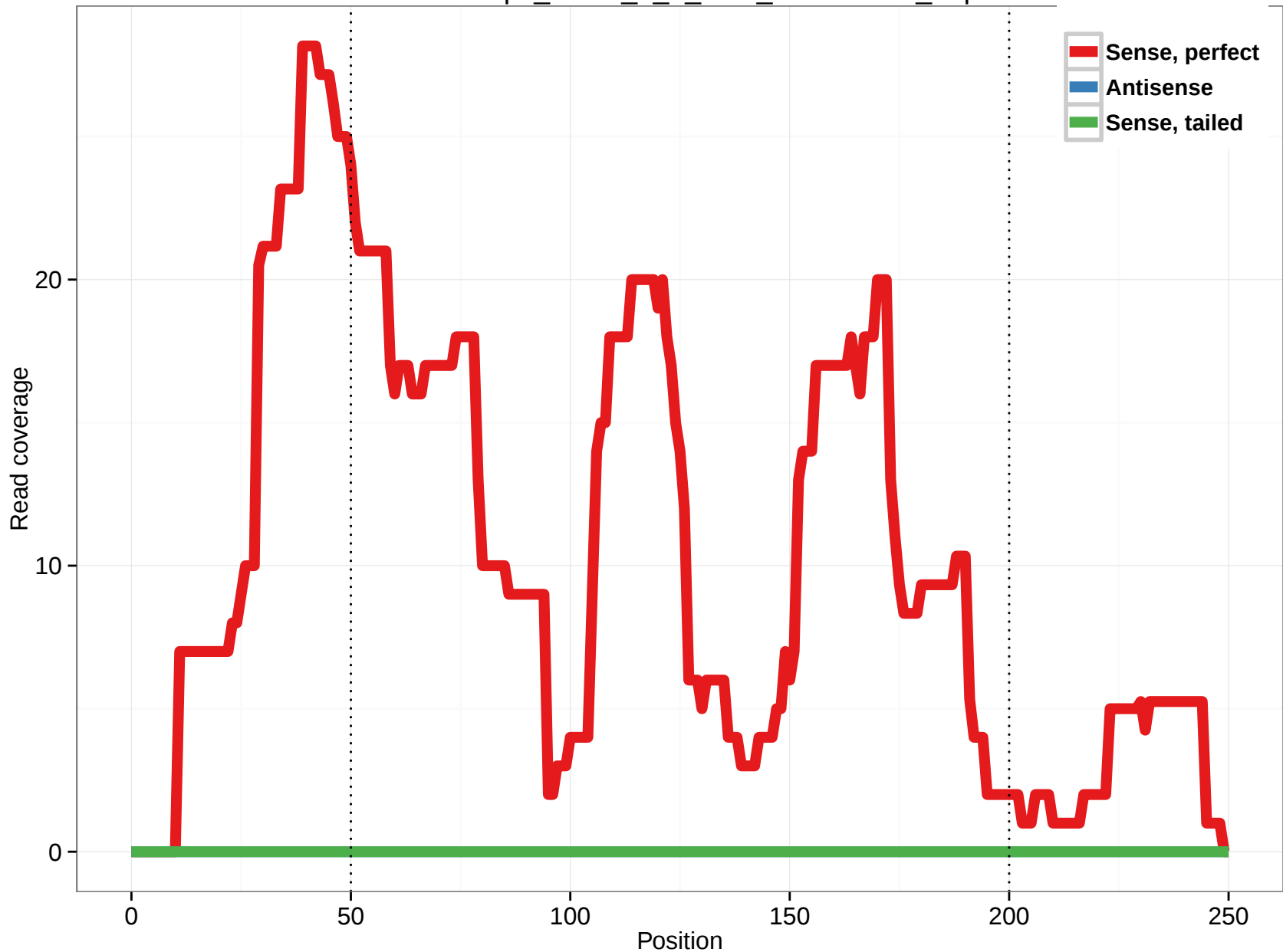
uc003ewq.1_intron_0_0_chr3_148749151_r.5p
