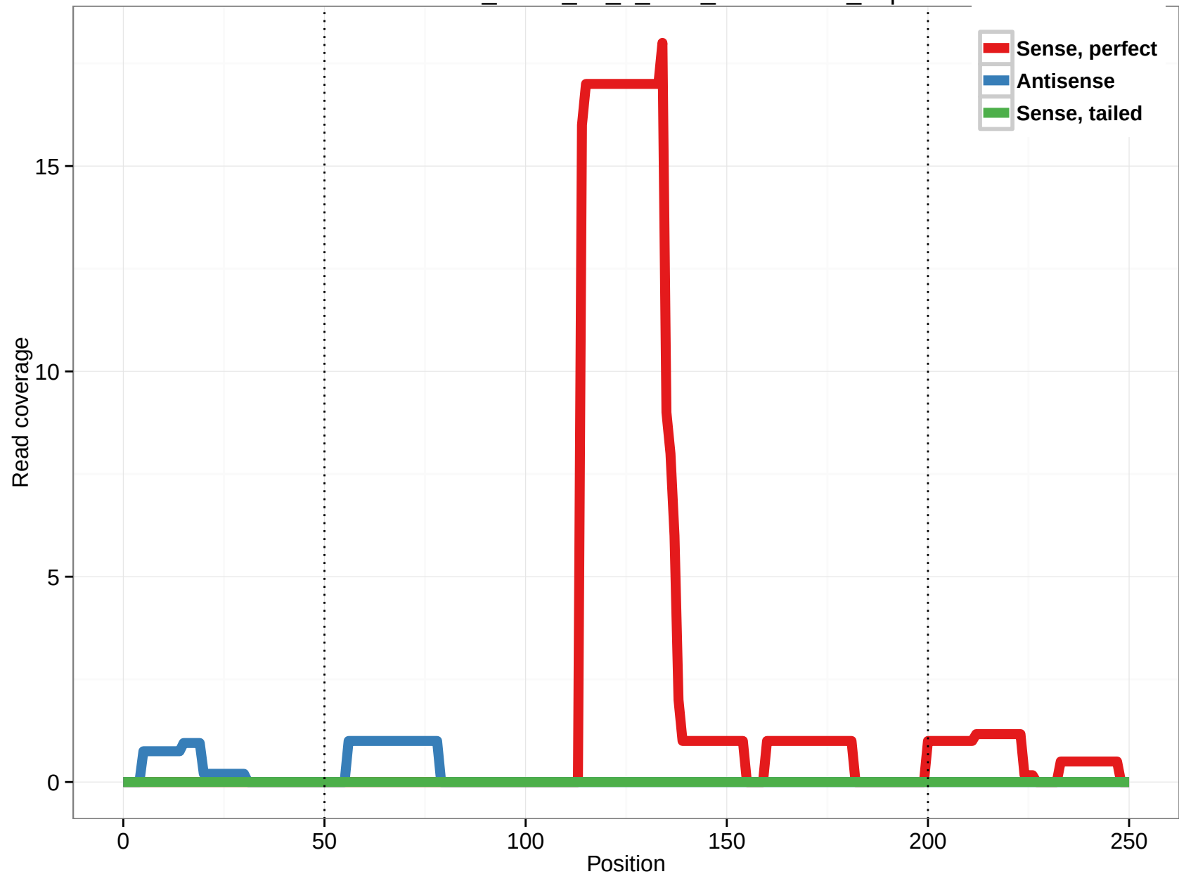
uc003esk.2_intron_18_0_chr3_138192477_f.3p
