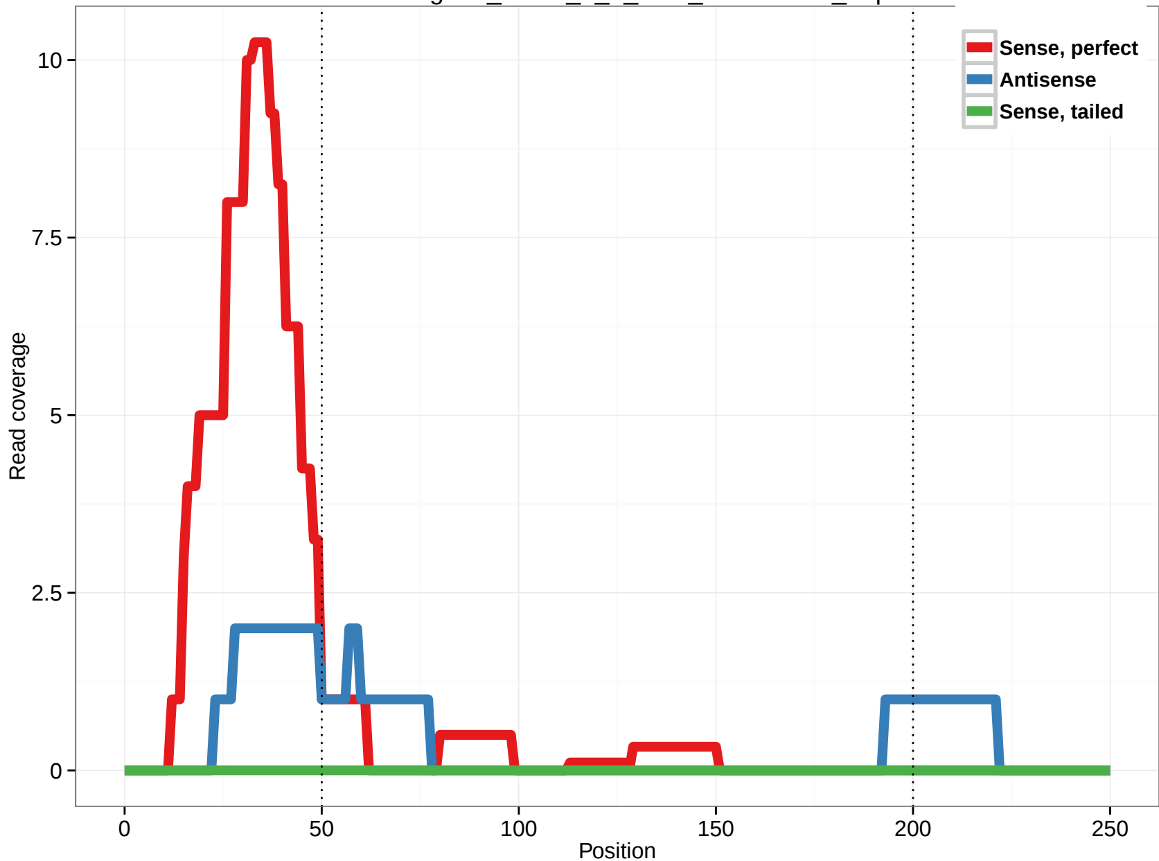
uc003egm.2_intron_1_0_chr3_123337615_r.5p
