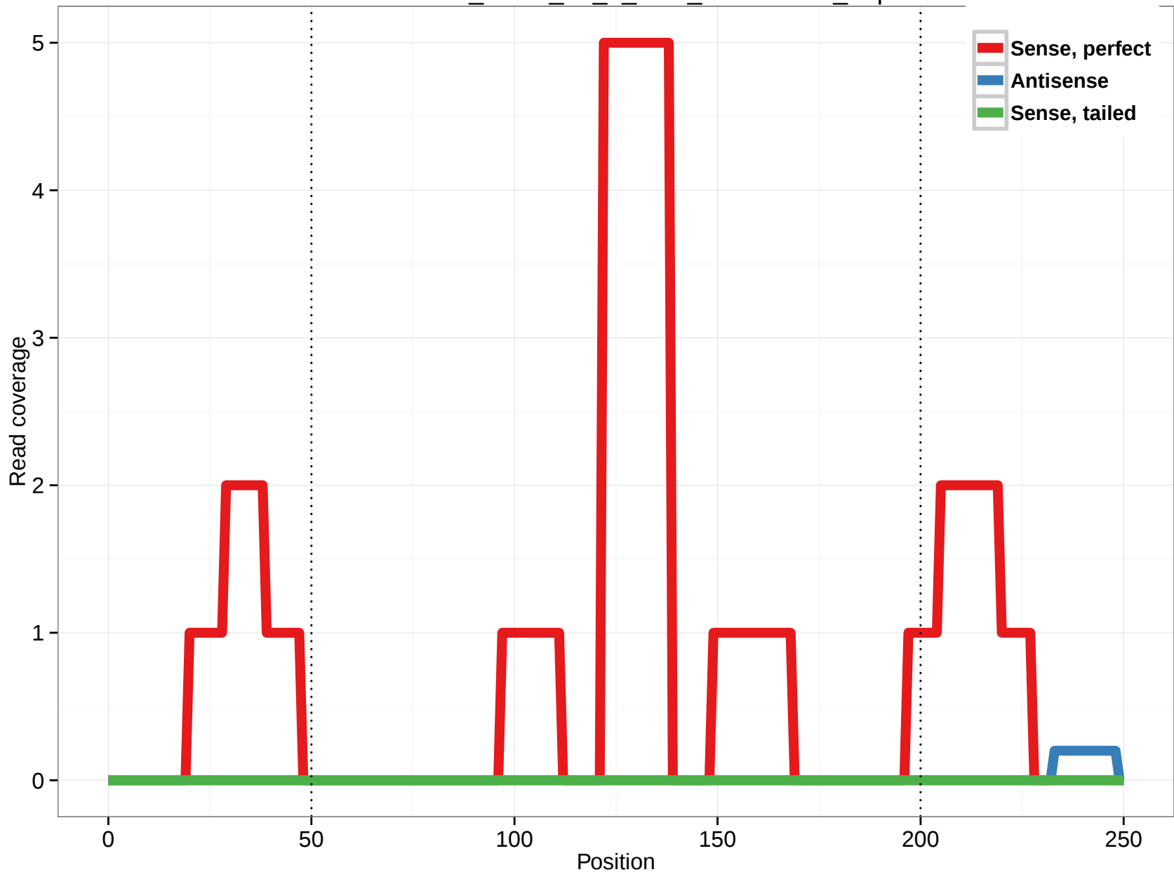
uc003eaf.3_intron_13_0_chr3_113212990_r.5p
