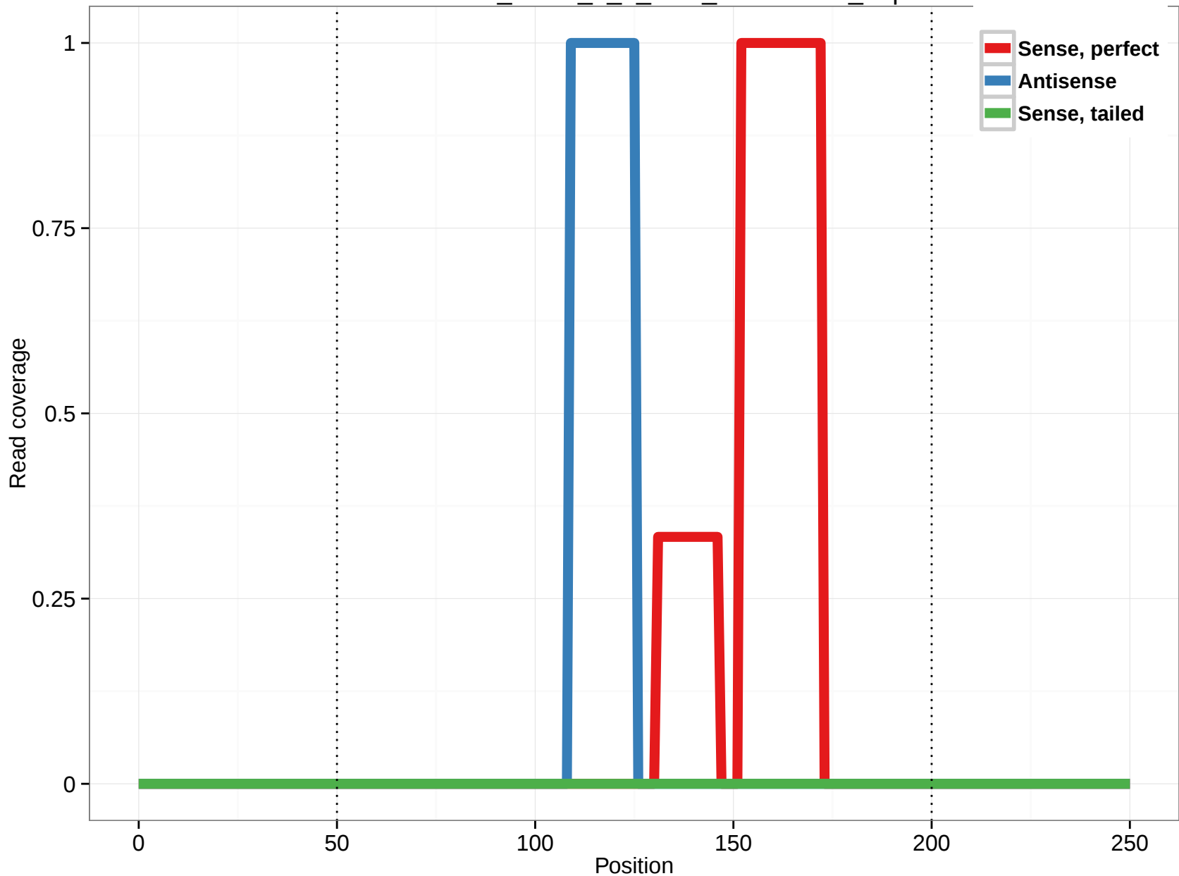
uc003dza.3_intron_2_0_chr3_112190203_r.5p
