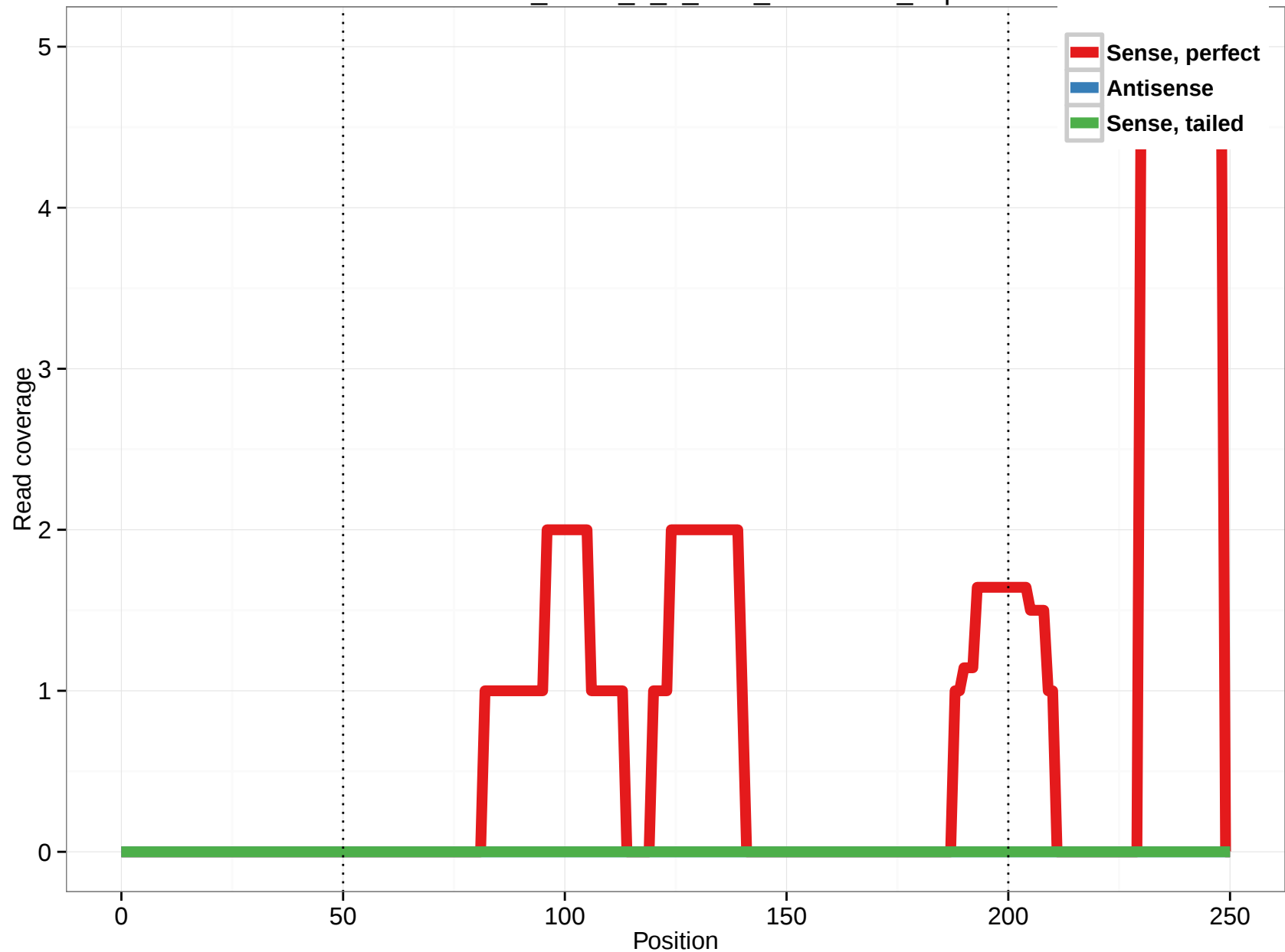
uc003dtk.1_intron_0_0_chr3_99536888_f.3p
