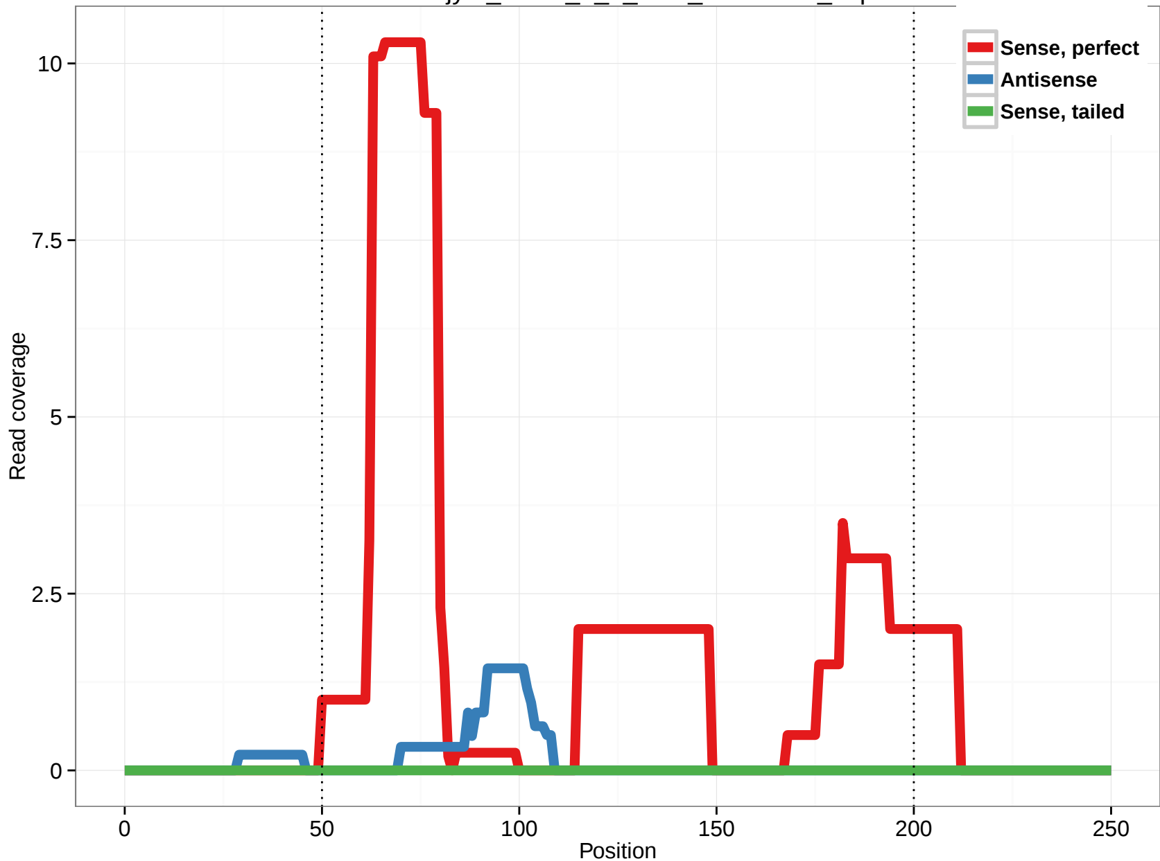
uc003dgy.1_intron_0_0_chr3_58318818_f.5p
