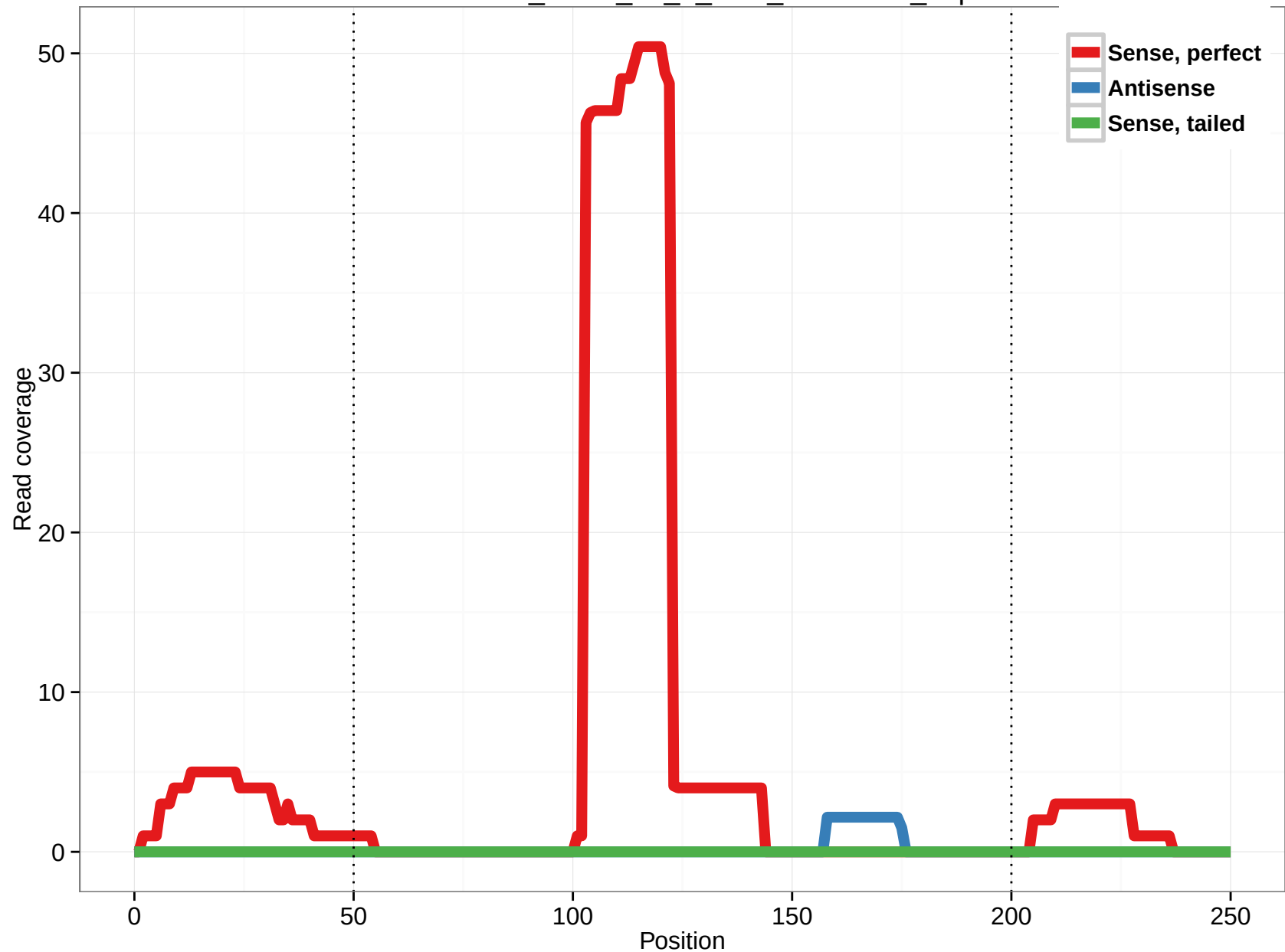
uc003dic.3_intron_14_0_chr3_56695046_r.5p
