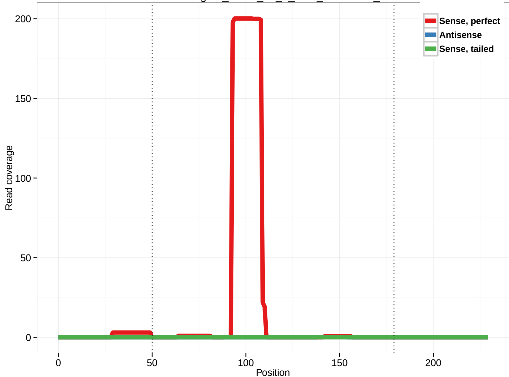
uc003dgu.3_intron_36_0_chr3_53810758_f
