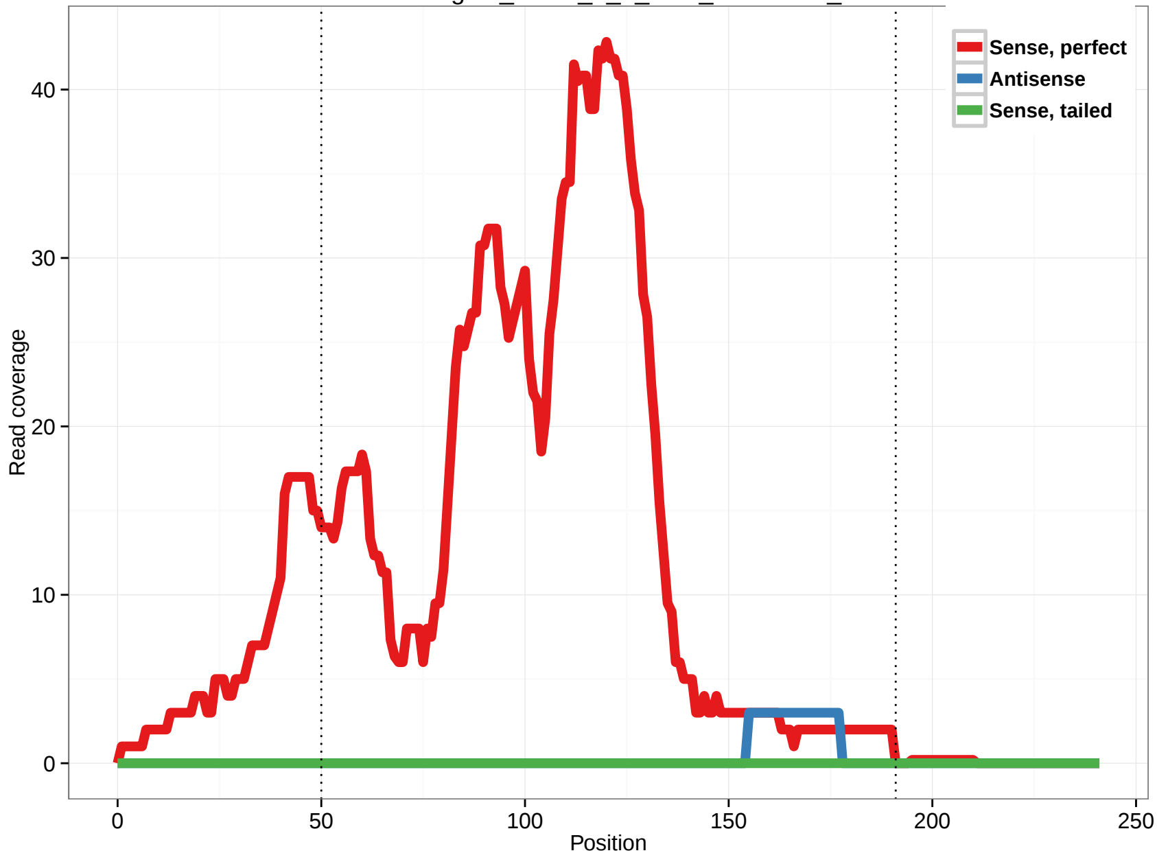
uc003dgo.2_intron_0_0_chr3_53259626_r
