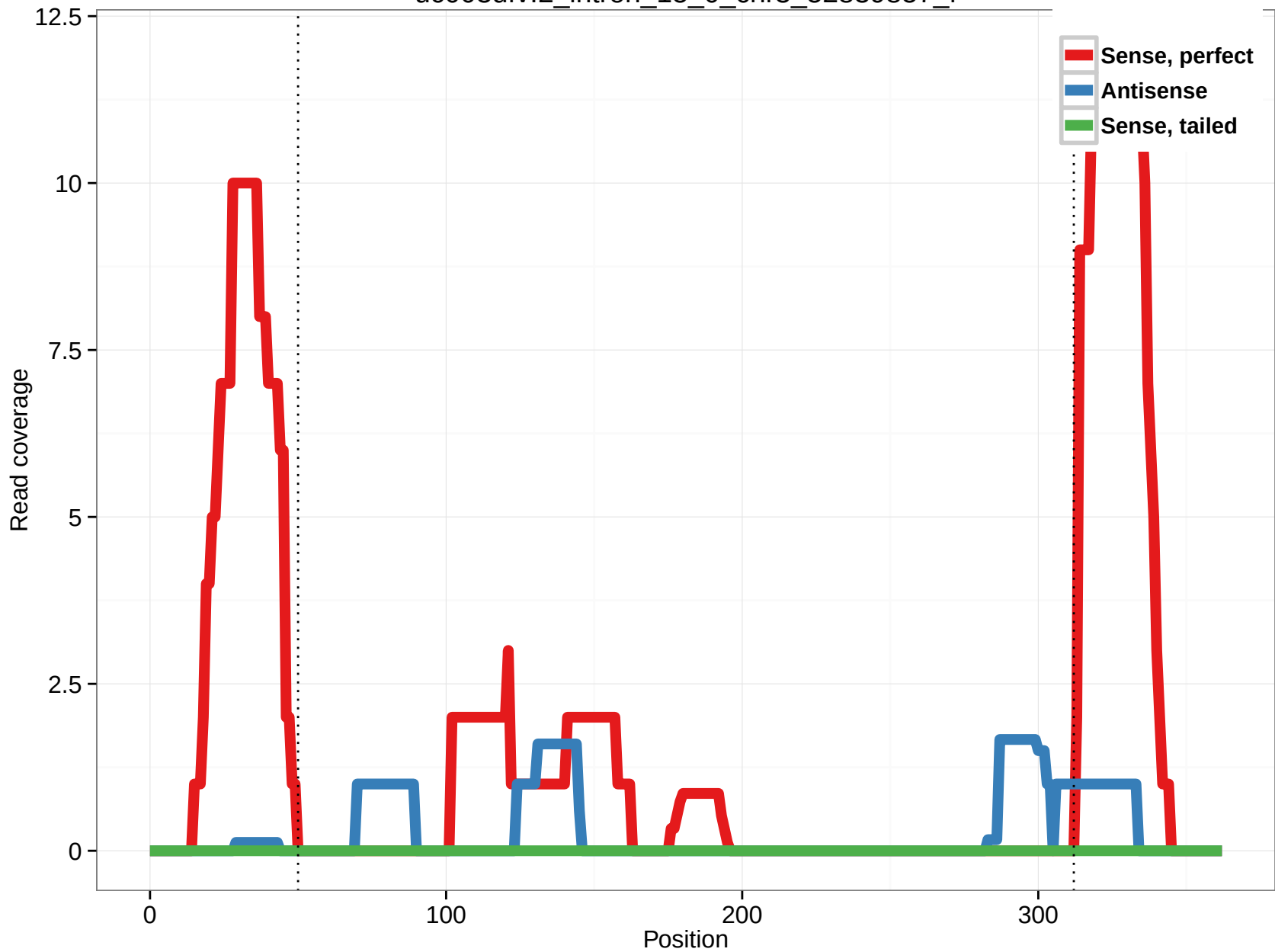
uc003dfv.2_intron_15_0_chr3_52839857_f
