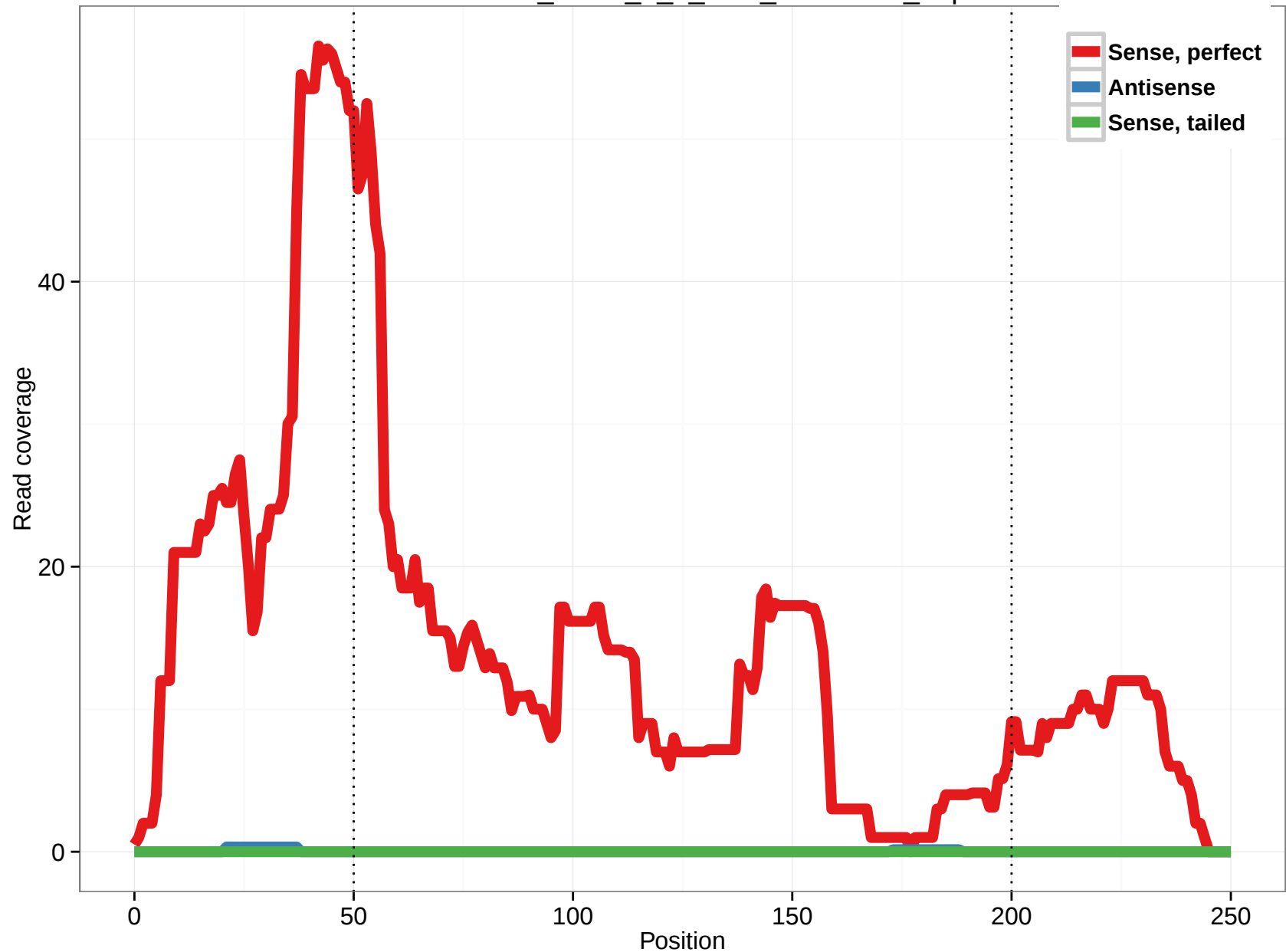
uc003dfk.2_intron_9_0_chr3_52738969_r.5p
