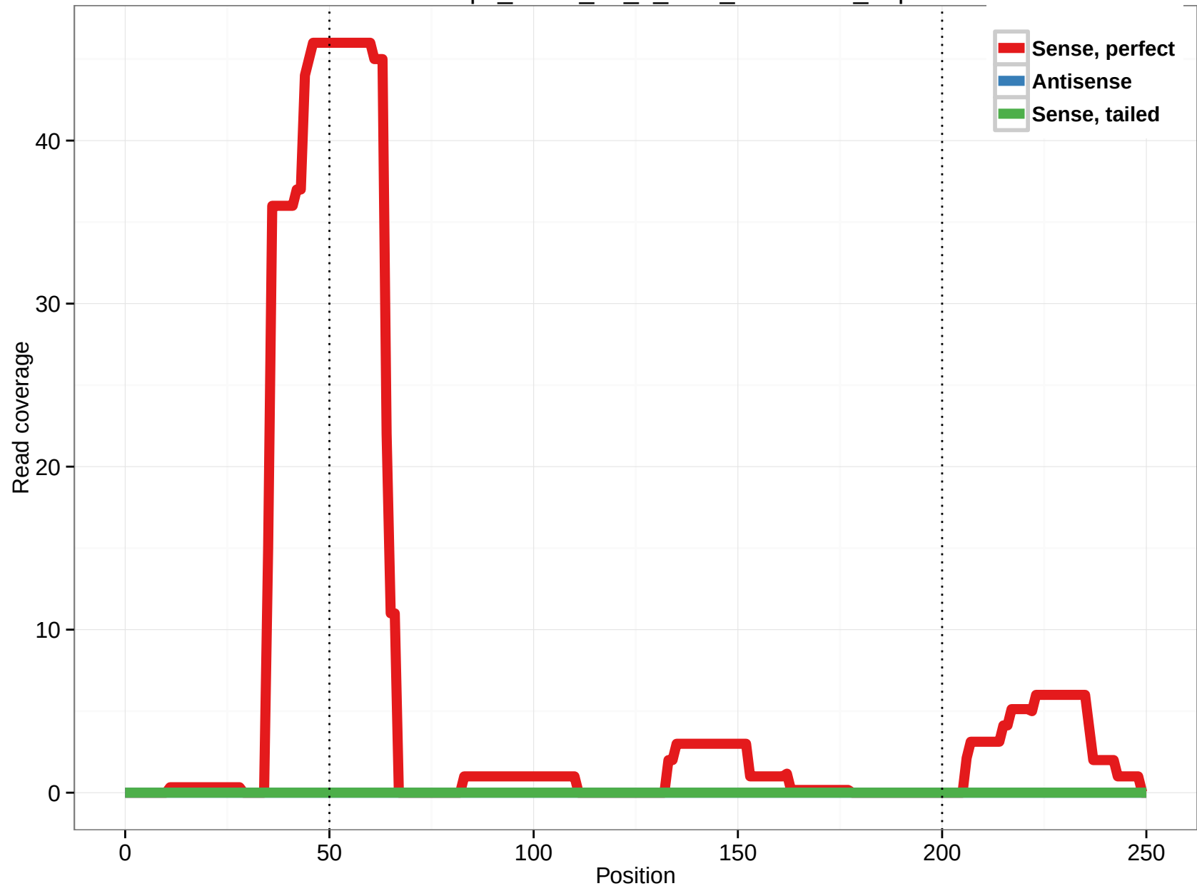
uc003deq.2_intron_10_0_chr3_52623272_r.3p
