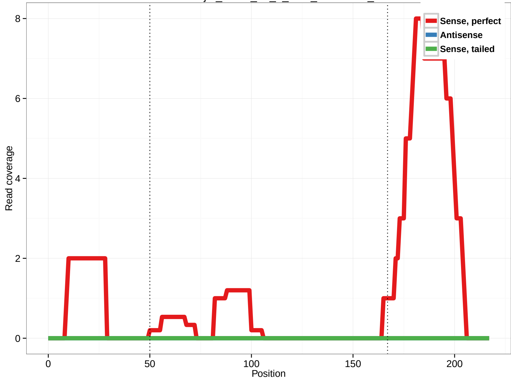
uc003dej.2_intron_37_0_chr3_52550255_f
