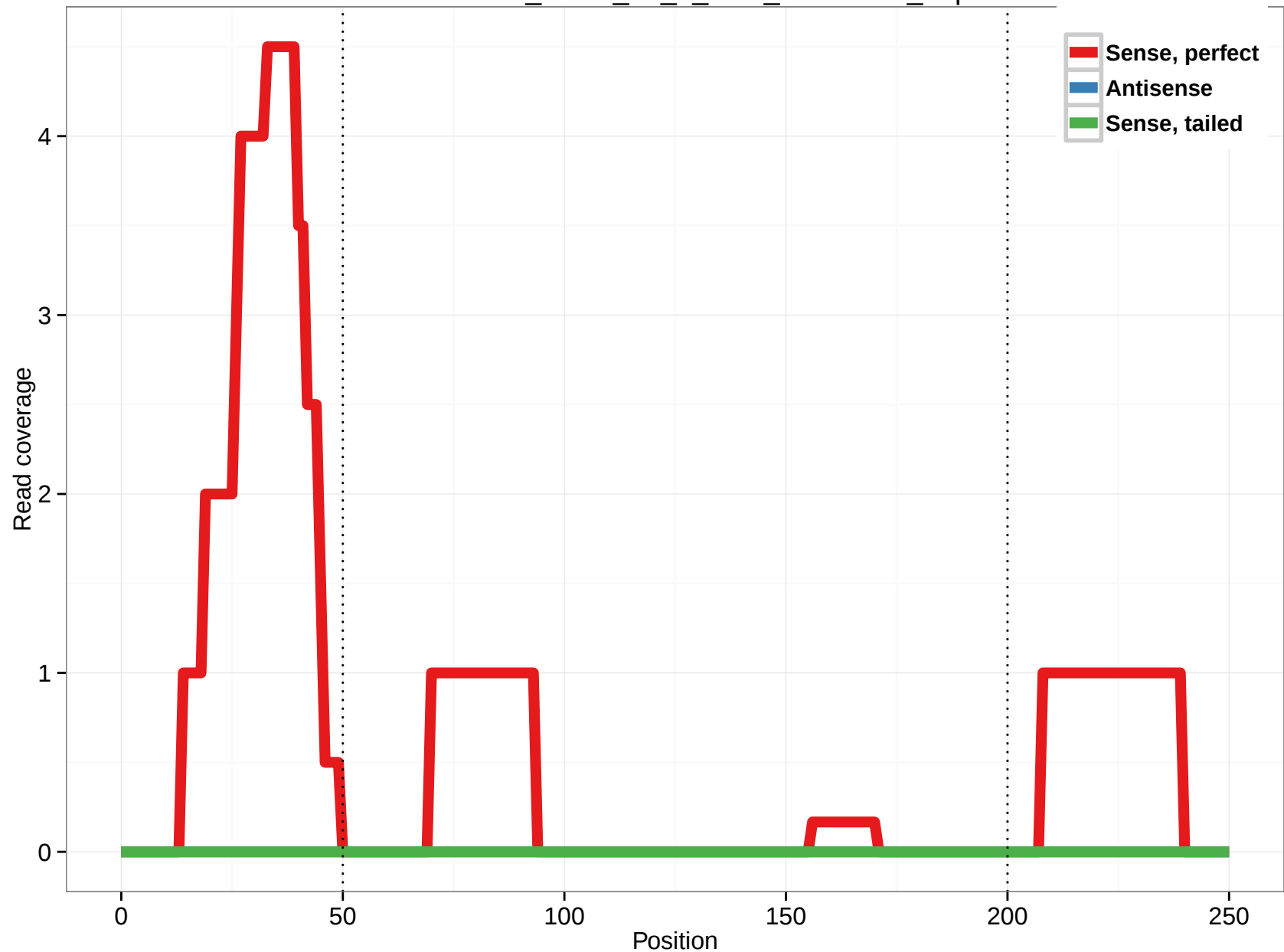
uc003csh.1_intron_11_0_chr3_48225327_r.5p
