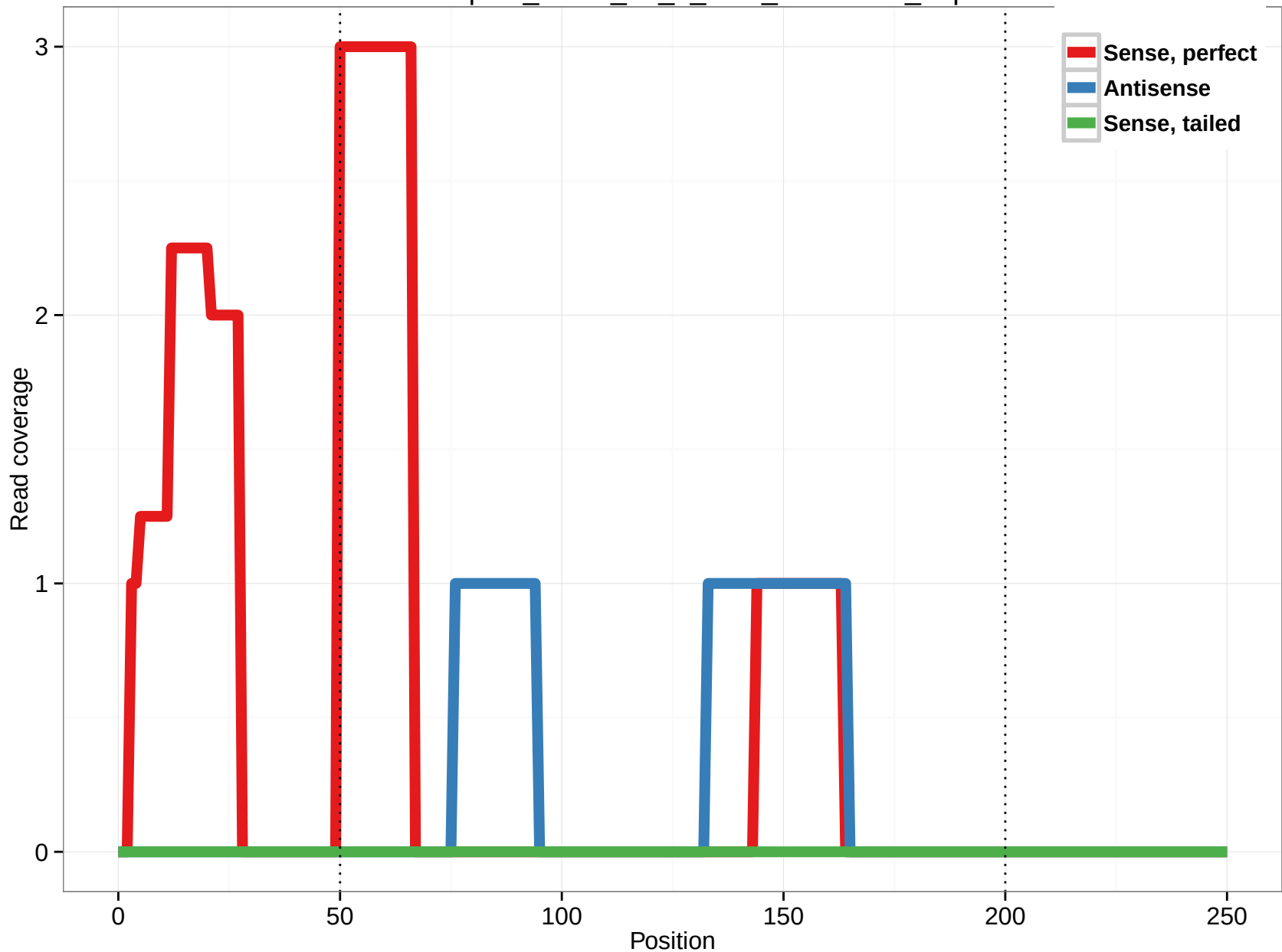
uc003cpb.3_intron_13_0_chr3_46016838_r.5p
