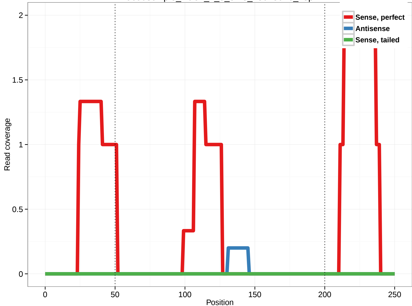
uc003cmp.3_intron_1_0_chr3_43075046_f.3p
