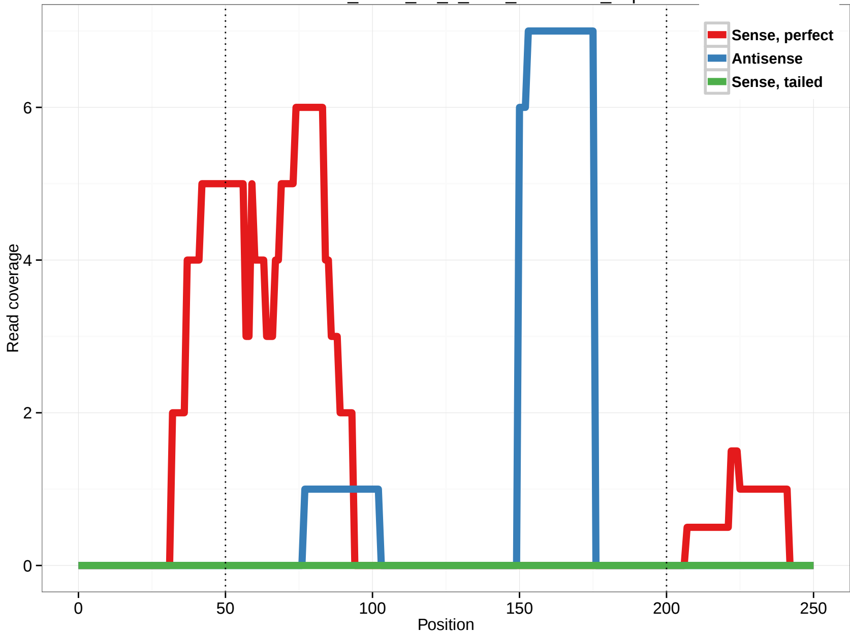
uc003chd.2_intron_25_0_chr3_37826570_f.3p
