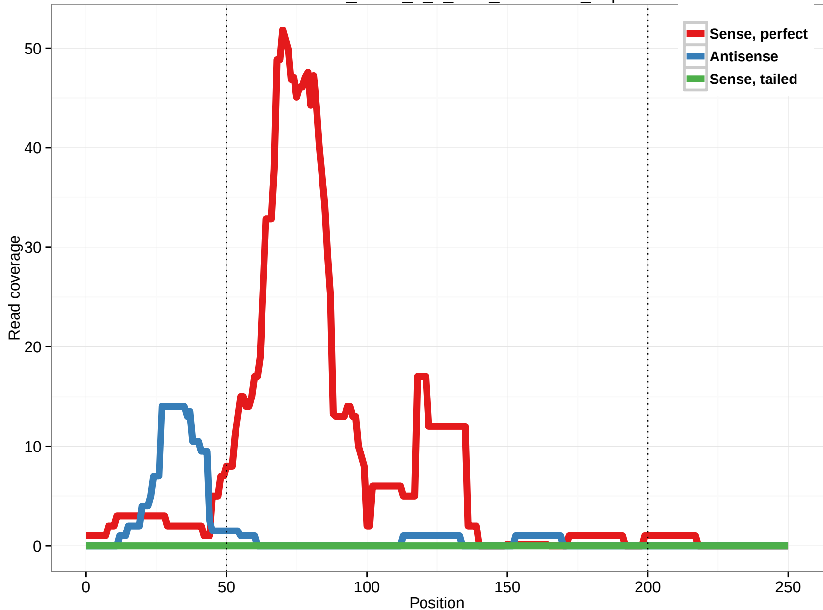
uc003ceb.2_intron_6_0_chr3_28382114_r.5p
