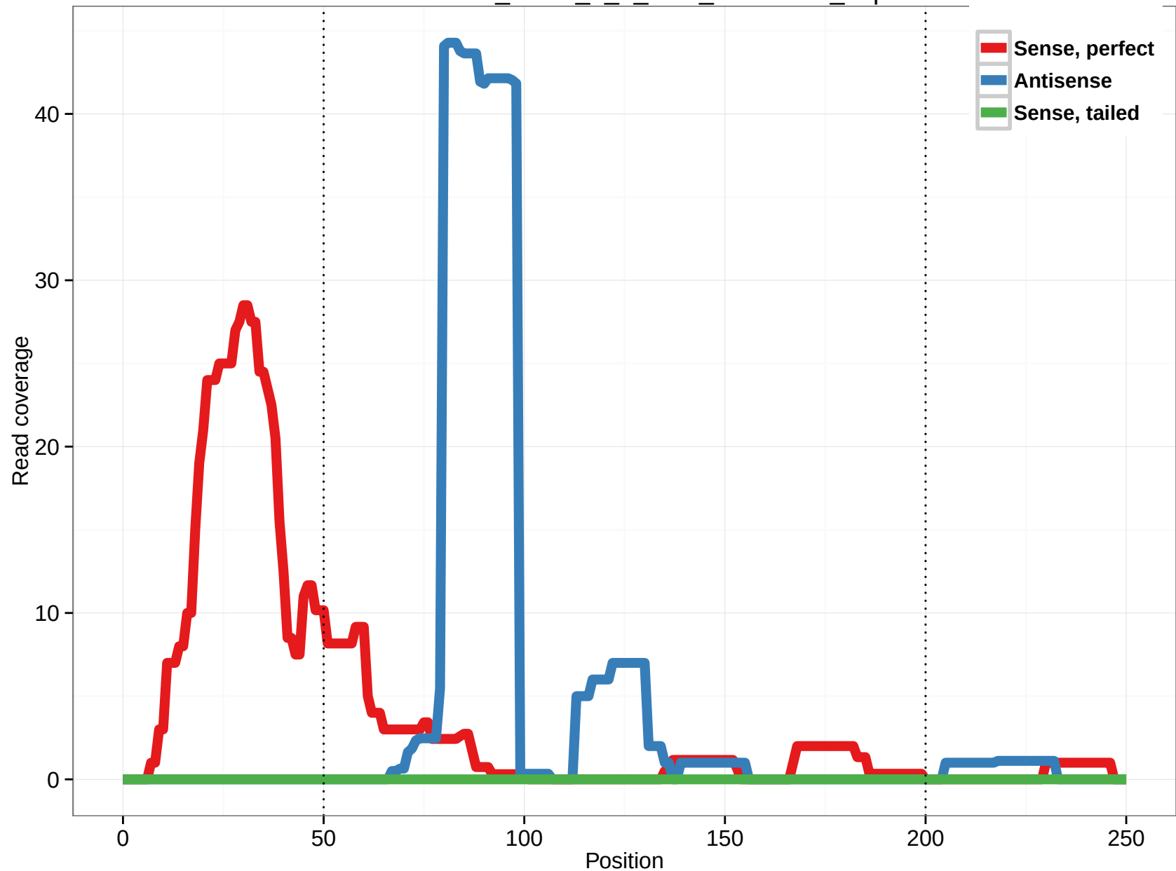
uc003cch.2_intron_0_0_chr3_23847580_f.5p
