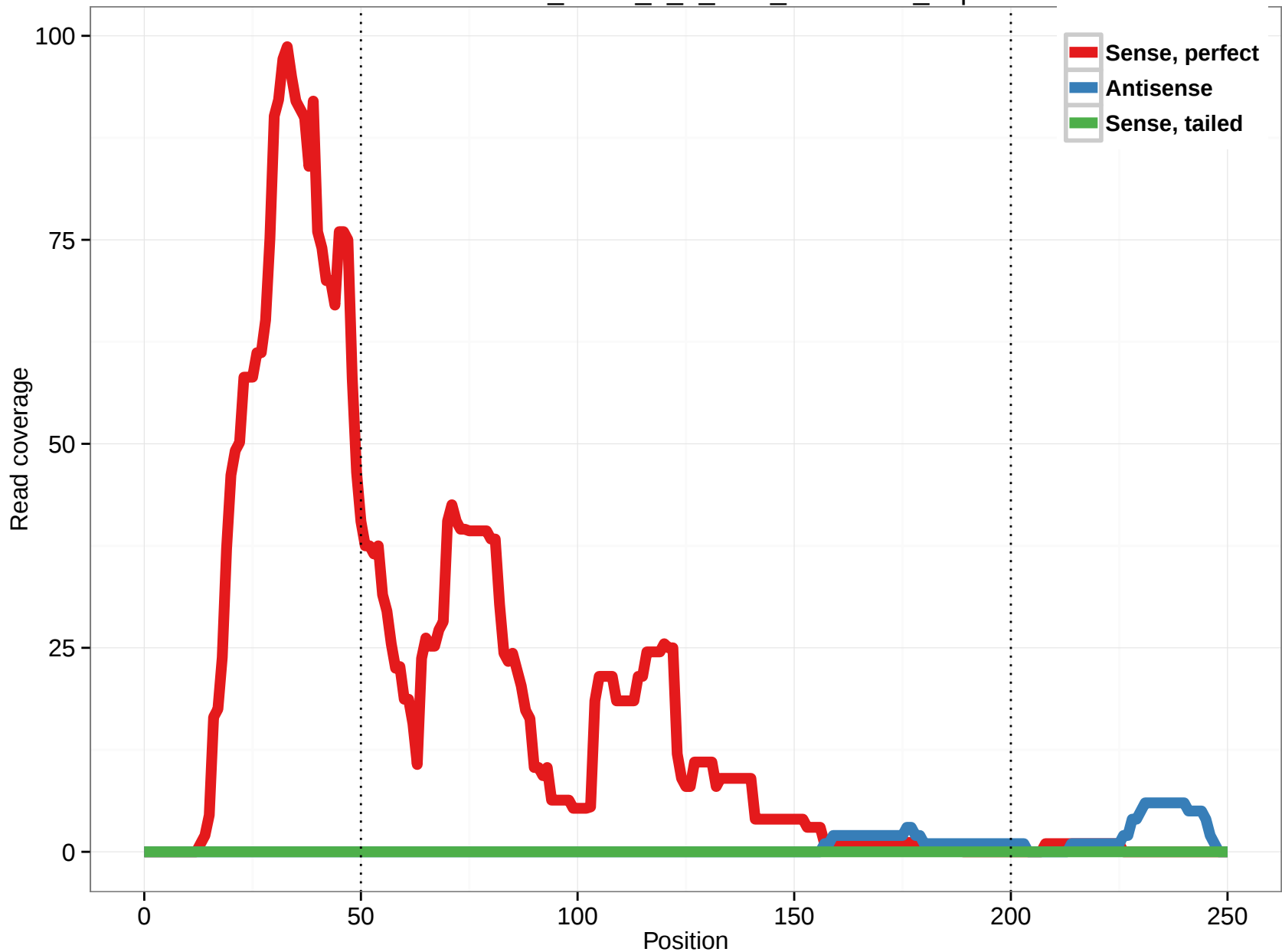
uc003bwc.2_intron_0_0_chr3_11314117_f.5p
