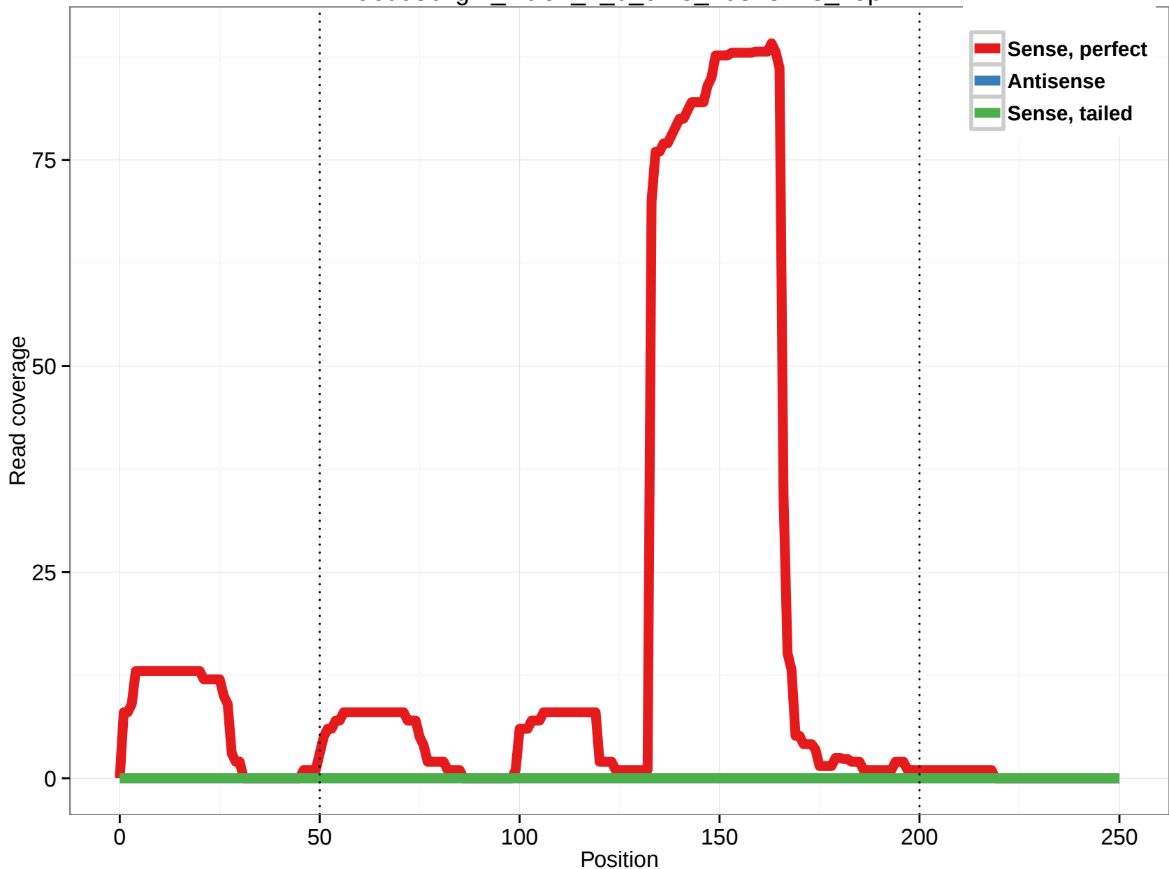
uc003bvg.2_intron_4_0_chr3_10318173_f.5p
