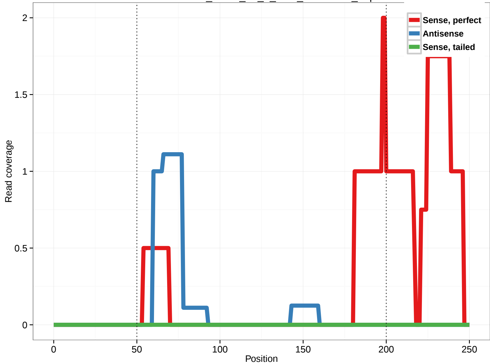
uc003buw.2_intron_17_0_chr3_10094182_f.3p
