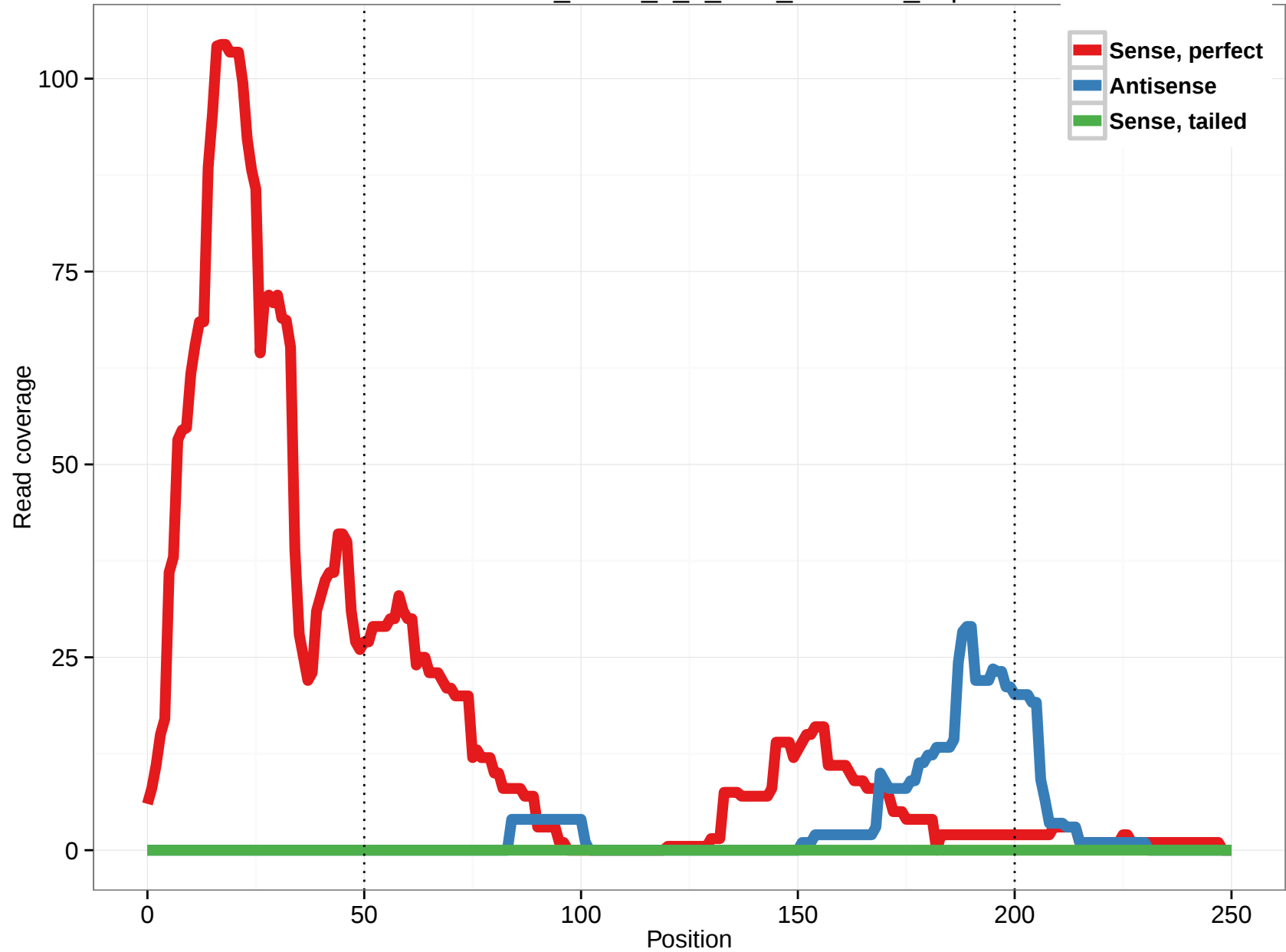
uc003bro.3_intron_0_0_chr3_9404812_f.5p
