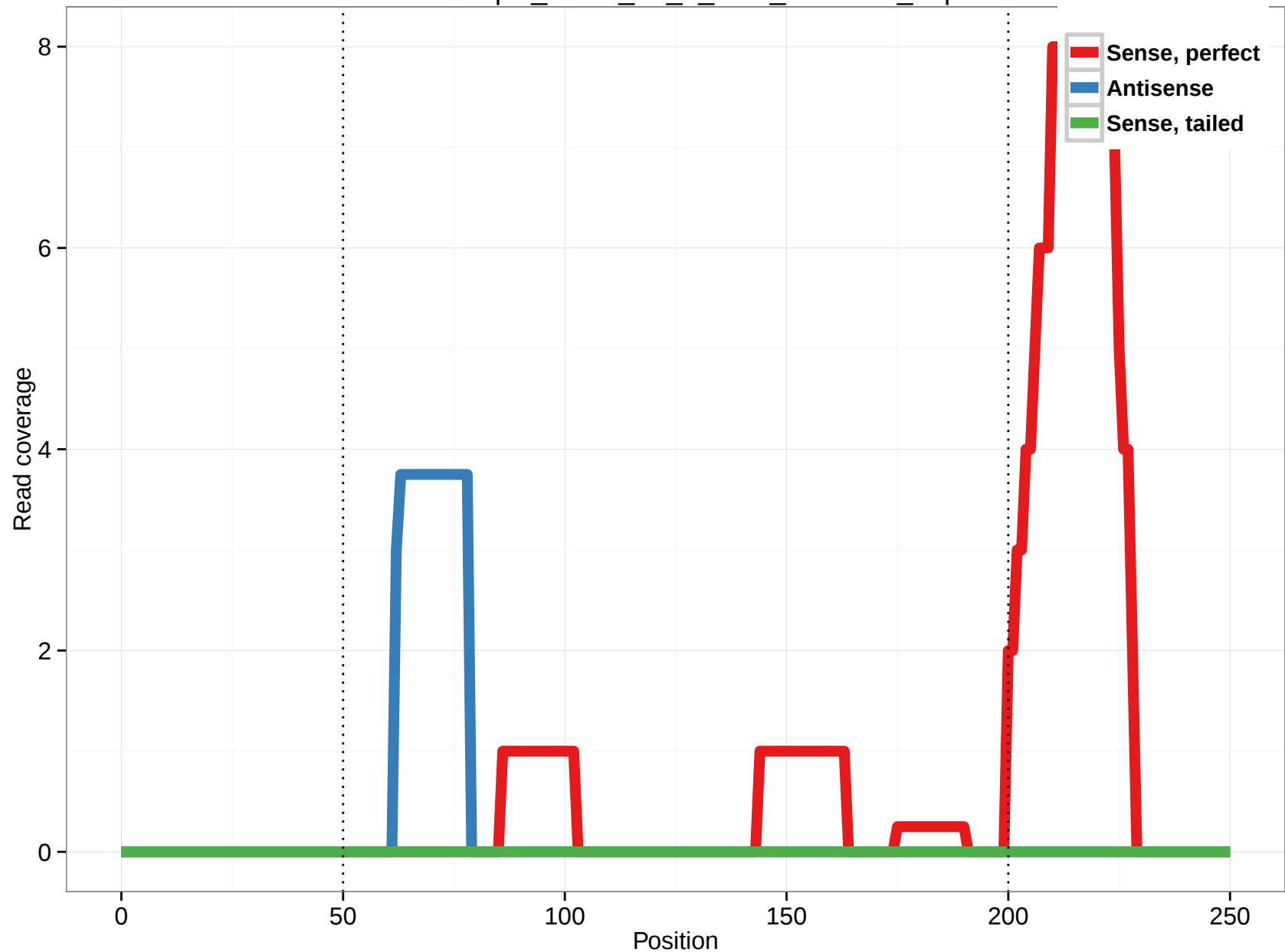
uc003bqi.2_intron_10_0_chr3_5255208_f.3p
