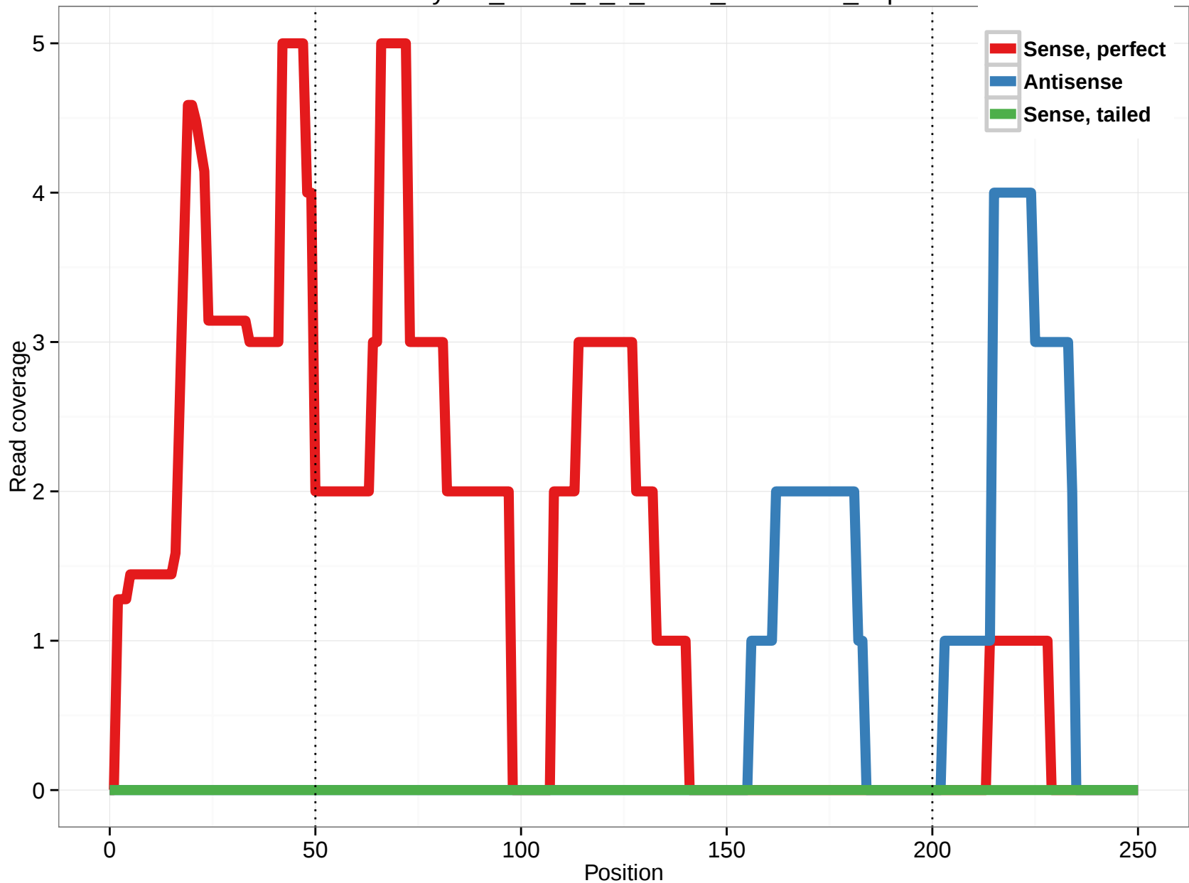
uc003aym.2_intron_4_0_chr22_40642107_f.5p
