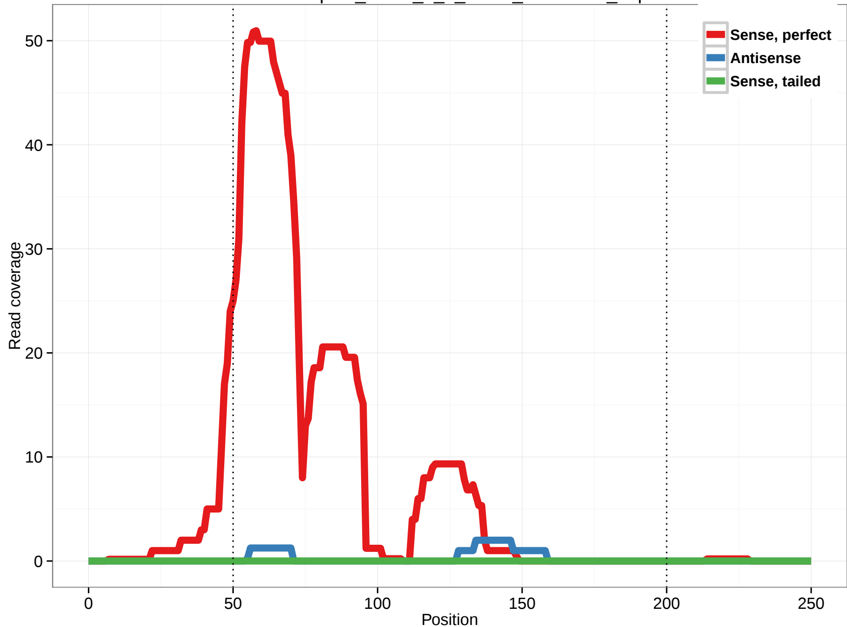
uc003aqm.2_intron_0_0_chr22_37415816_f.5p
