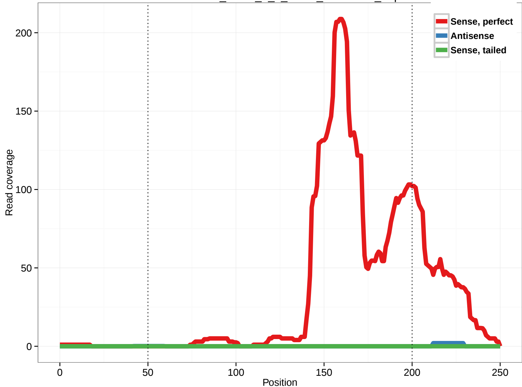
uc003aob.2_intron_2_0_chr22_36013313_r.3p
