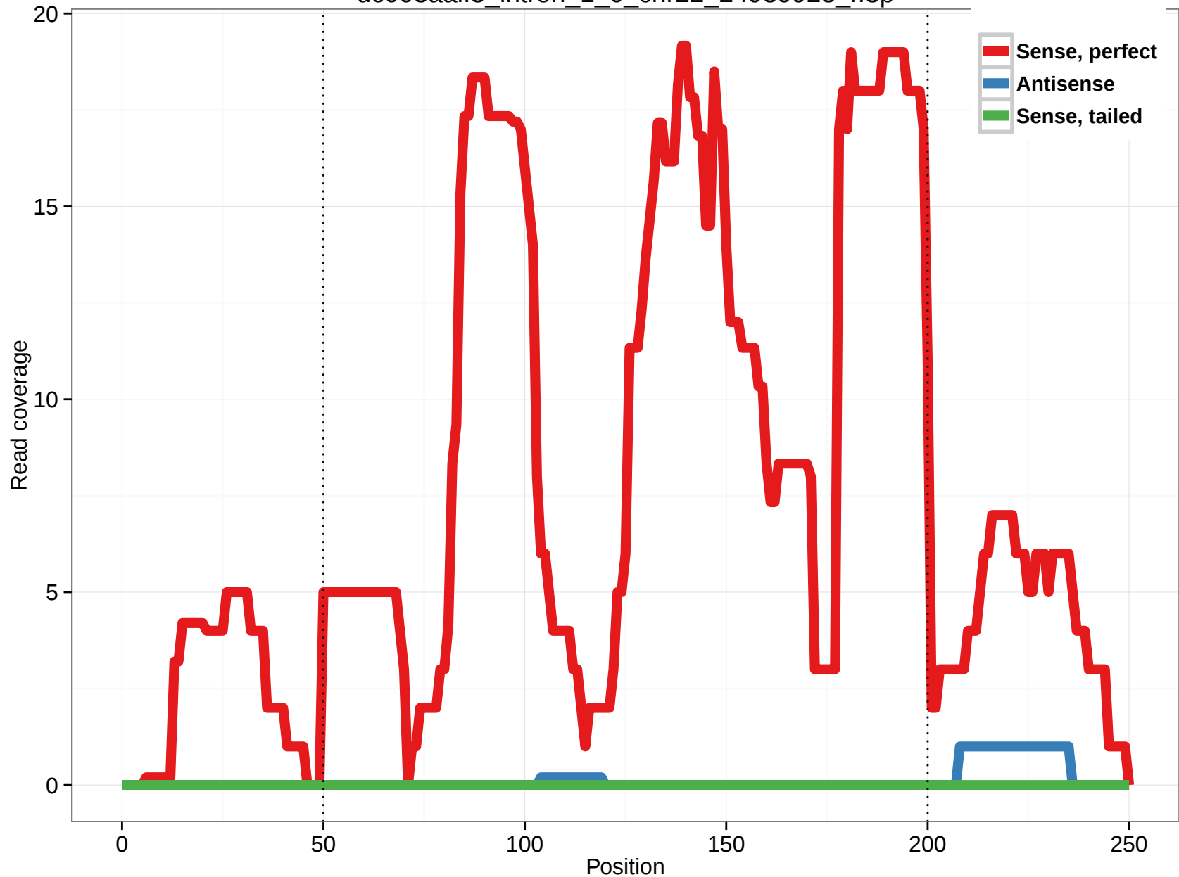
uc003aai.3_intron_1_0_chr22_24939923_r.3p
