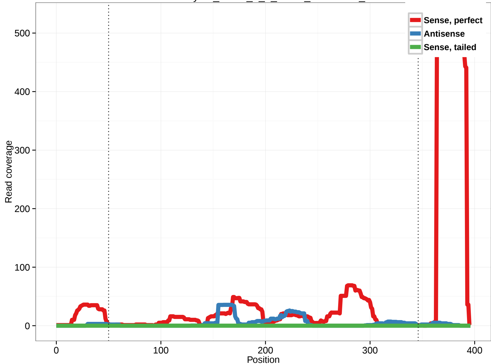
uc002zys.1_intron_0_0_chr22_24237720_r
