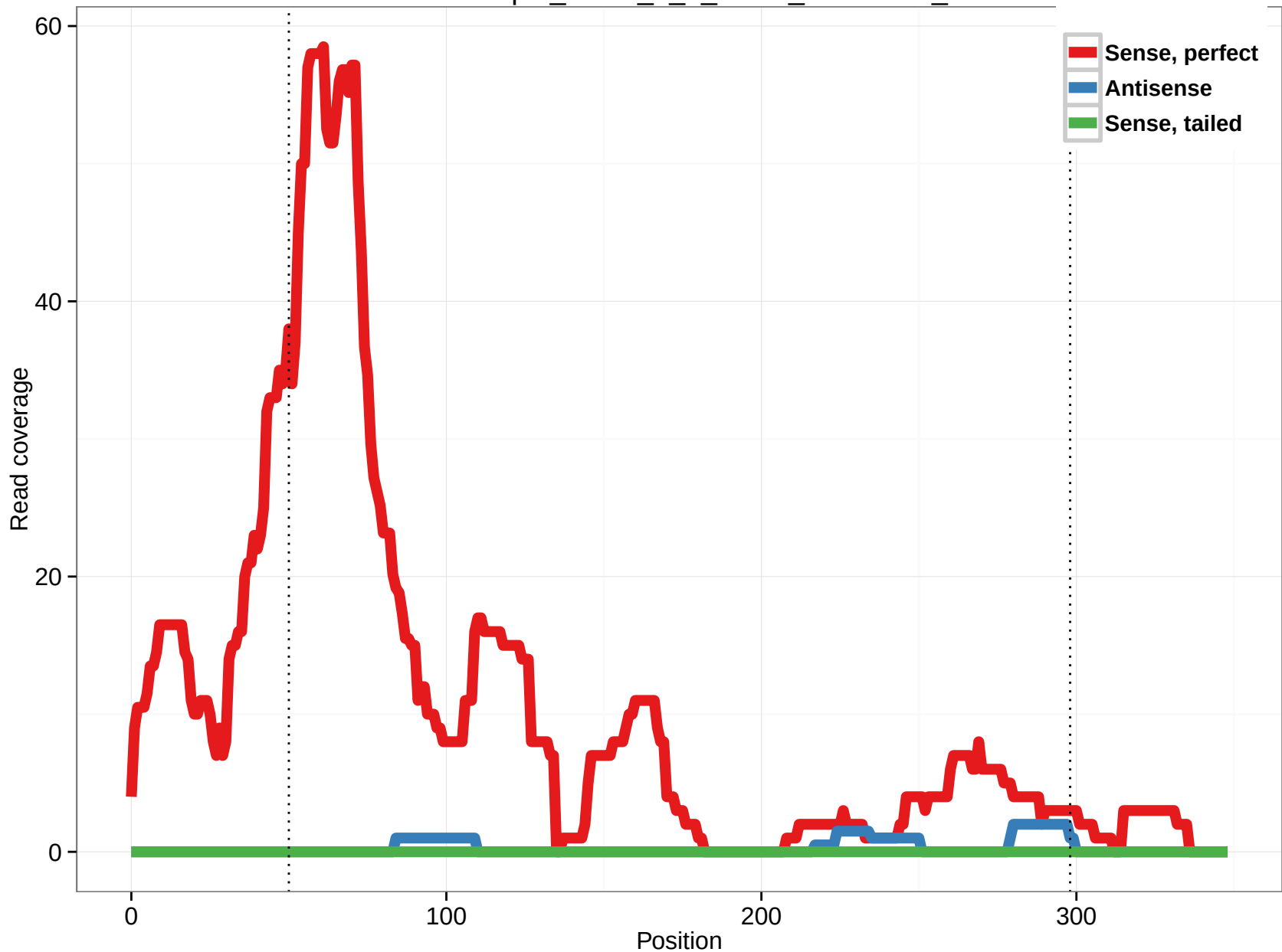
uc002znp.3_intron_0_0_chr22_18560814_f
