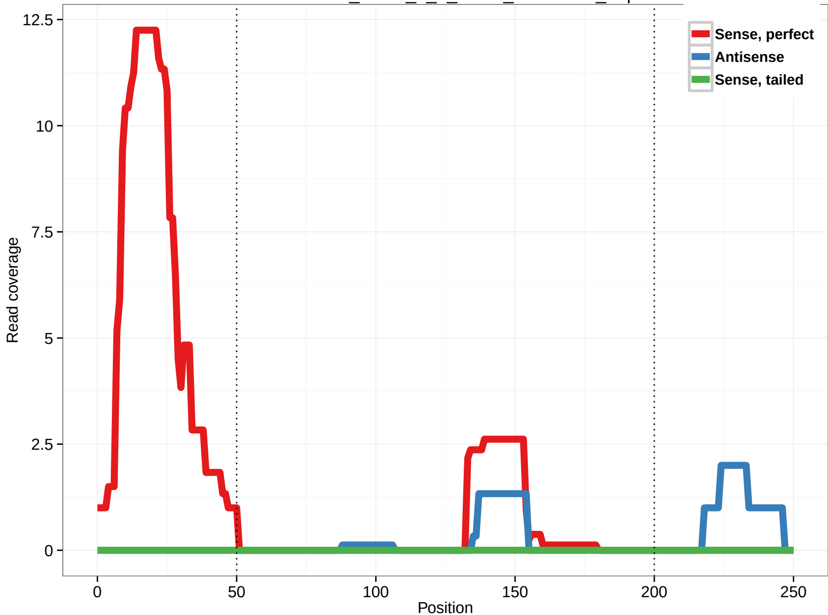
uc002zmr.1_intron_2_0_chr22_18081055_r.5p
