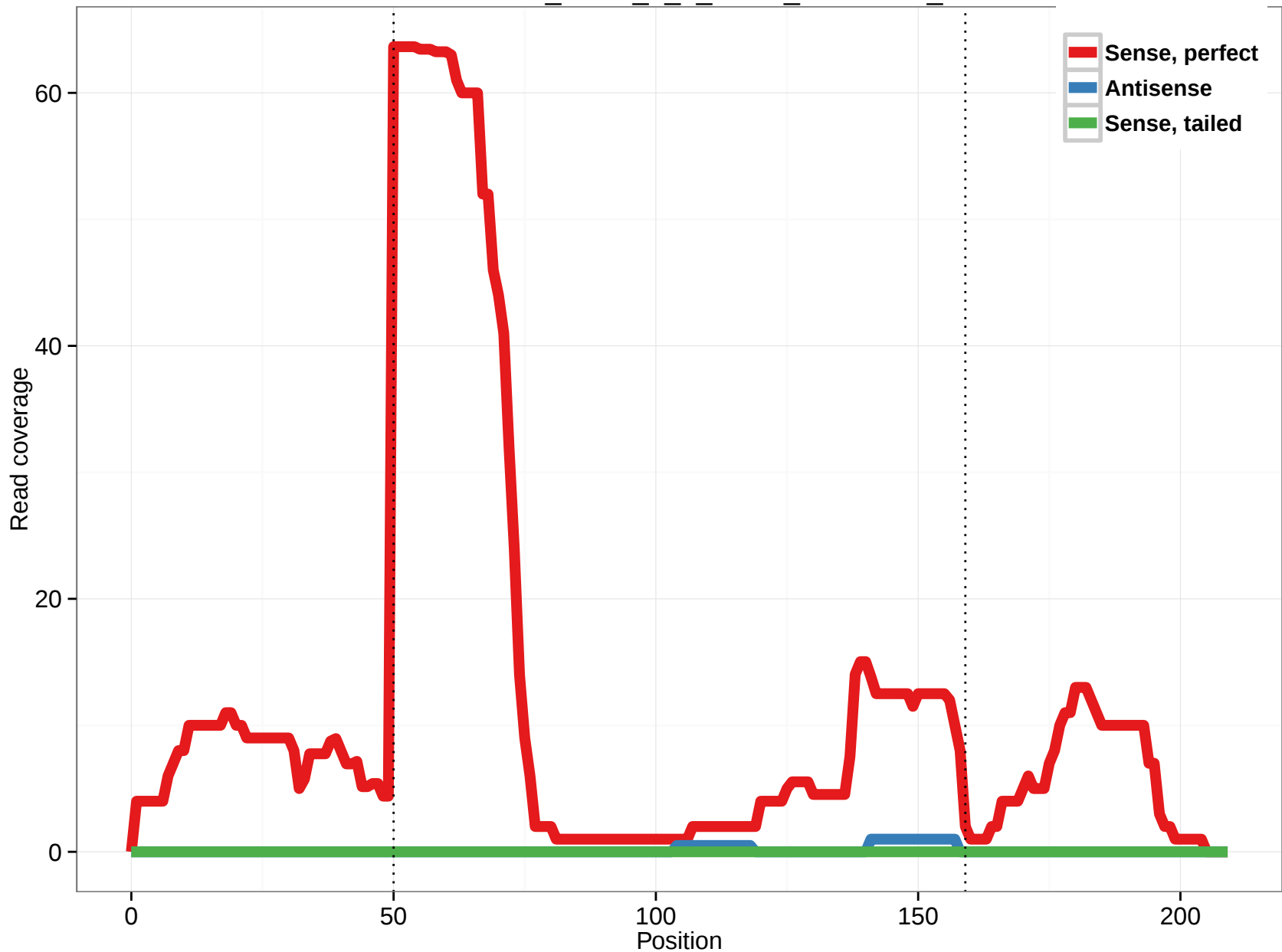
uc002zdf.2_intron_7_0_chr21_44841014_r
