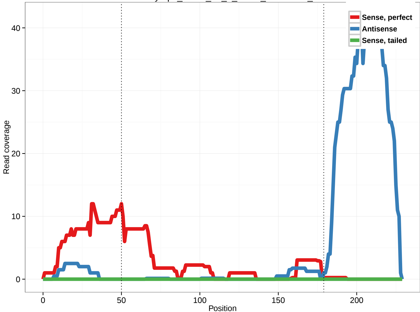
uc002yzq.1_intron_29_0_chr21_43299250_r
