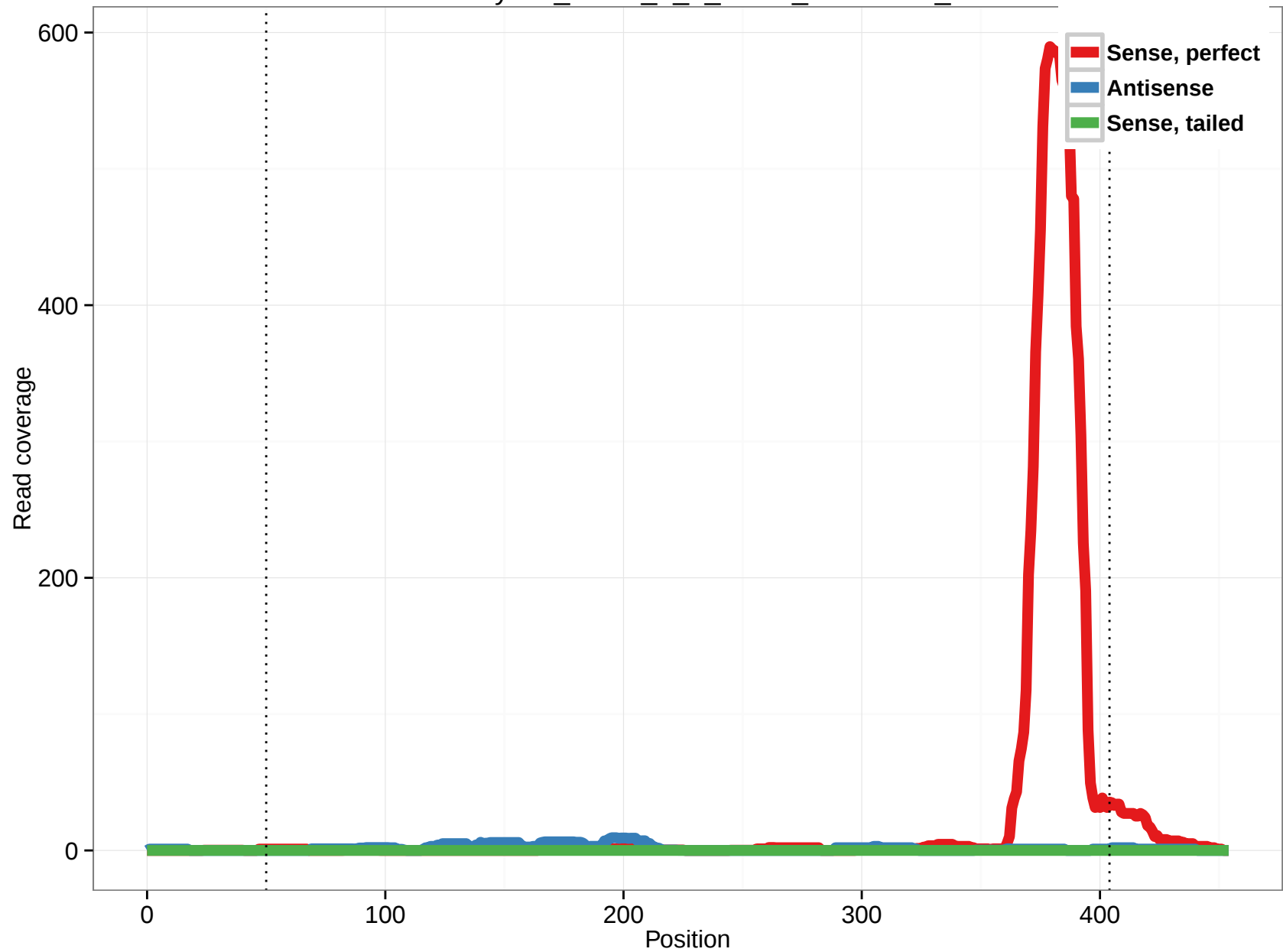
uc002yxf.2_intron_0_0_chr21_40177541_f
