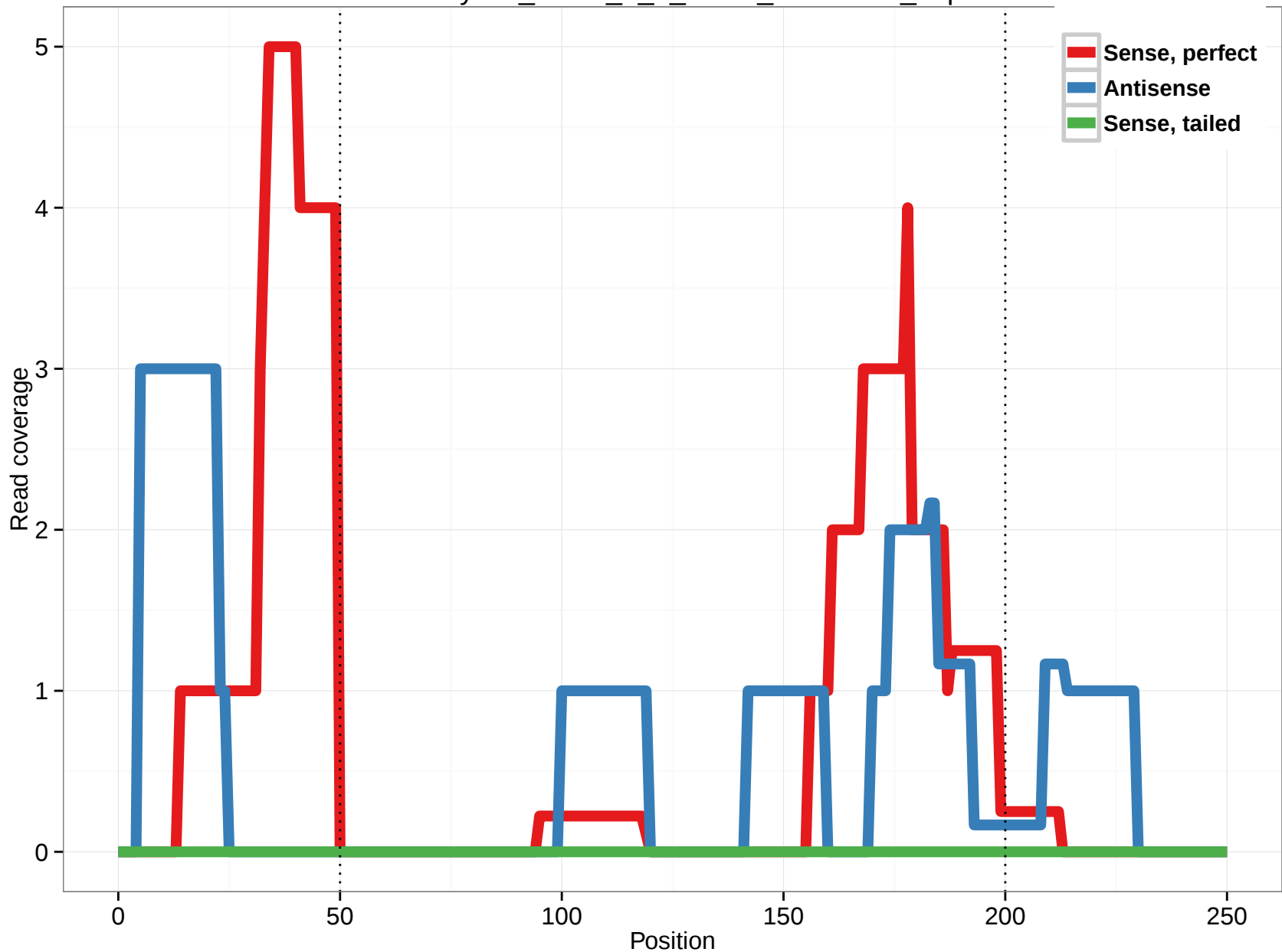
uc002yvi.2_intron_1_0_chr21_37706017_f.5p
