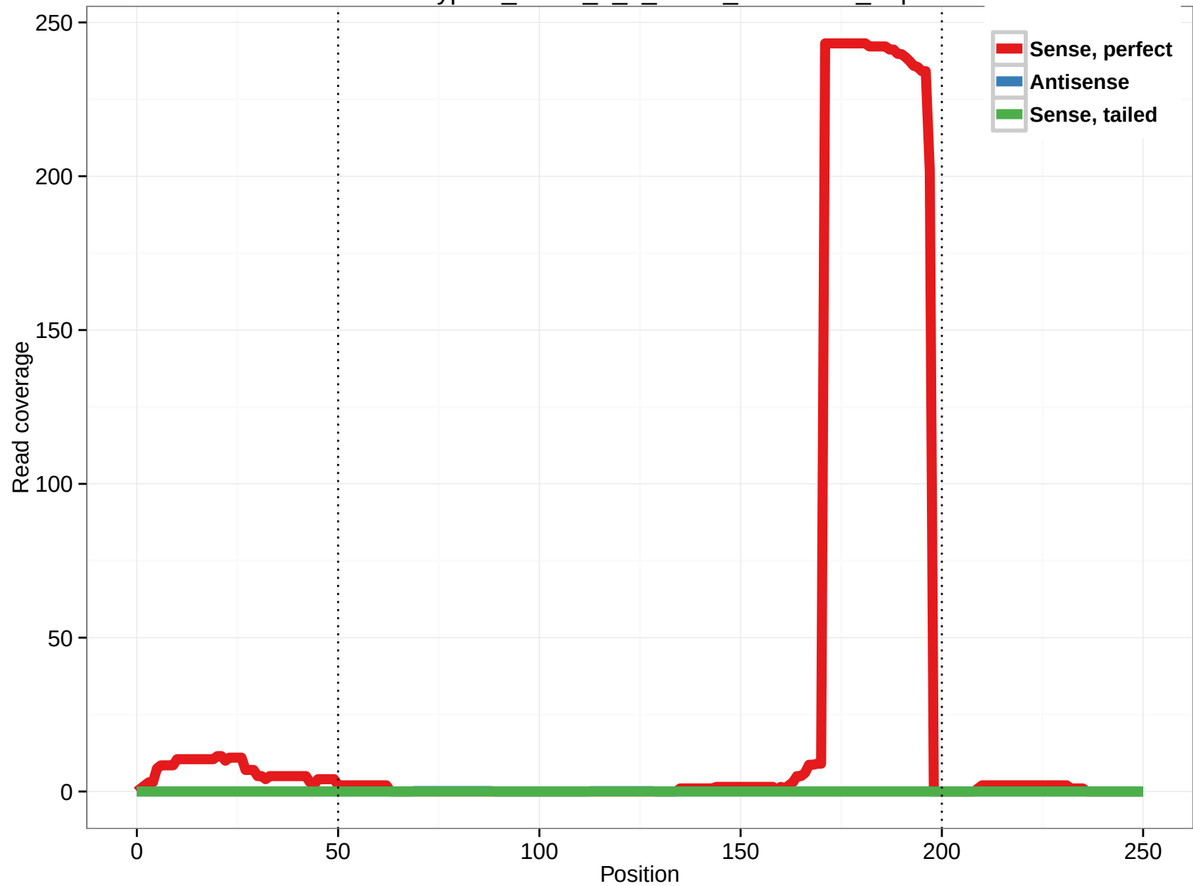
uc002ypd.2_intron_5_0_chr21_33063267_r.5p
