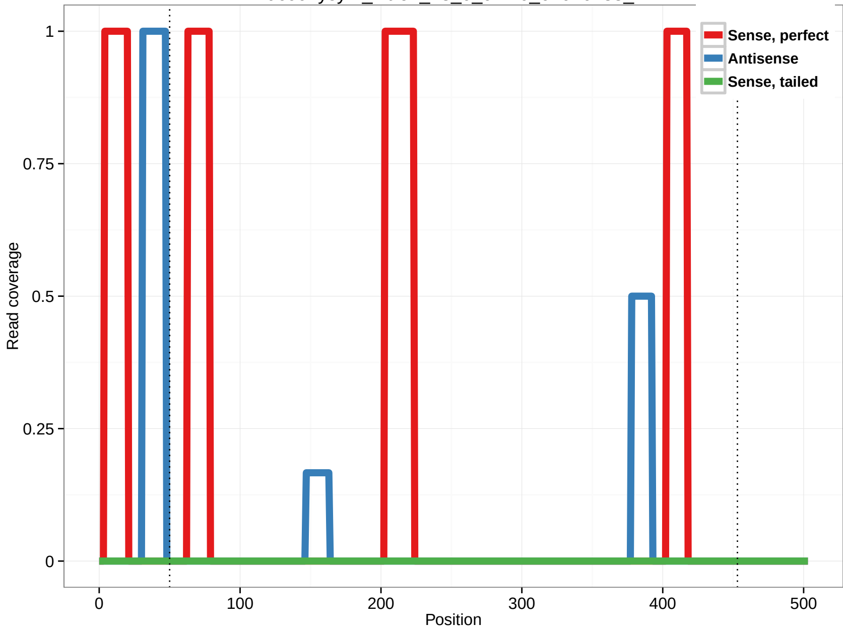
uc002yey.1_intron_13_0_chr20_62076188_r
