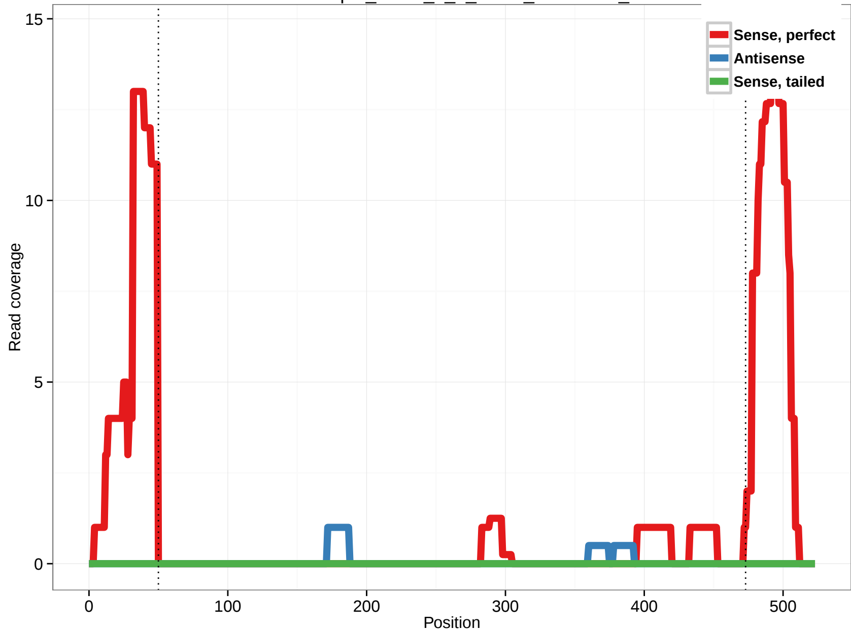
uc002xzp.2_intron_2_0_chr20_57273830_f
